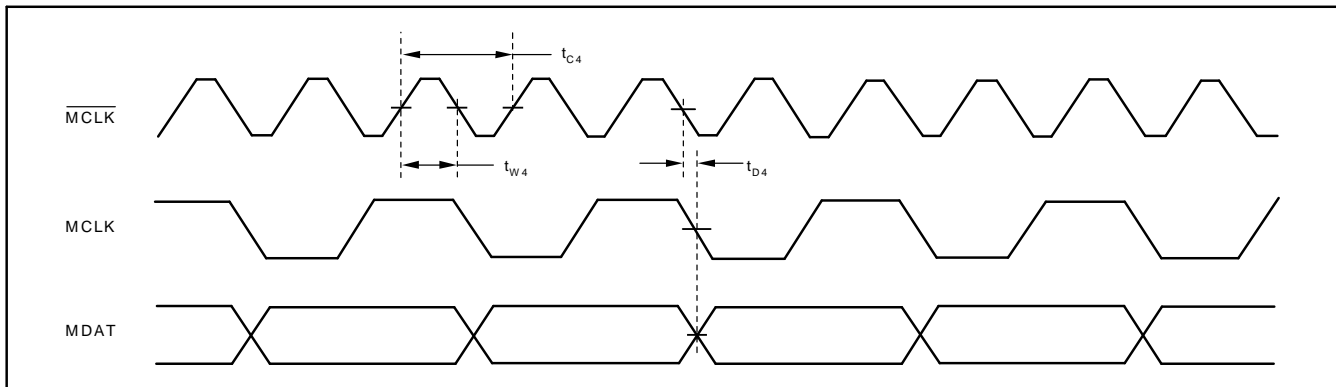
Figure 4. Mode 3 Operation
