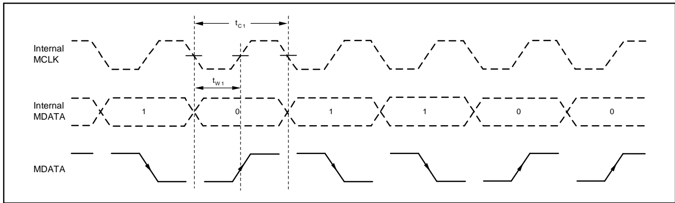
Figure 3. Mode 2 Operation
