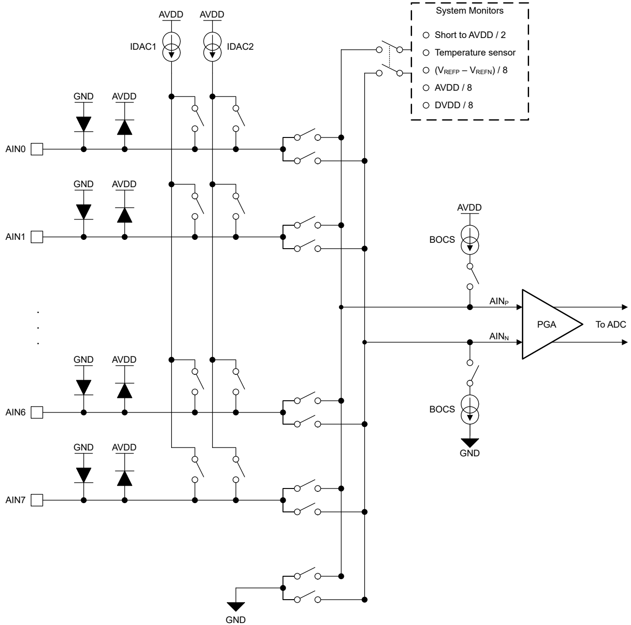
Figure 7-1. Input Multiplexer
