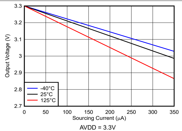
Figure 5-5. GPIO Pin Output Voltage vs Sourcing Current
