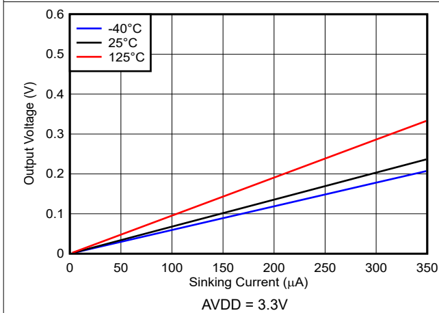
Figure 5-4. GPIO Pin Output Voltage vs Sinking Current
