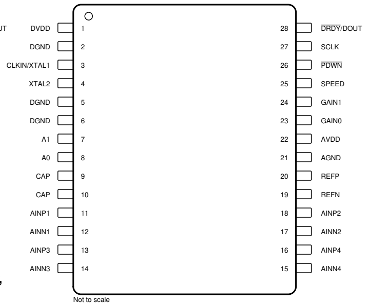
Figure 5-2. ADS1234 PW Package, 28-Pin TSSOP, Top View
