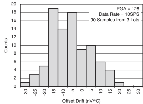
Figure 6-14. Offset Drift ( 25^\circ\text{C} to 105^\circ\text{C} )
