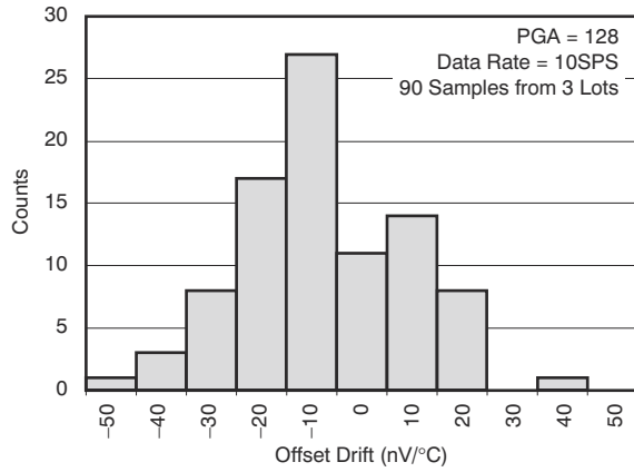
Figure 6-13. Offset Drift ( -40^\circ\text{C} to +25^\circ\text{C} )
