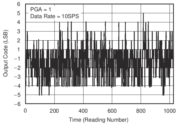
Figure 6-1. Noise Plot
