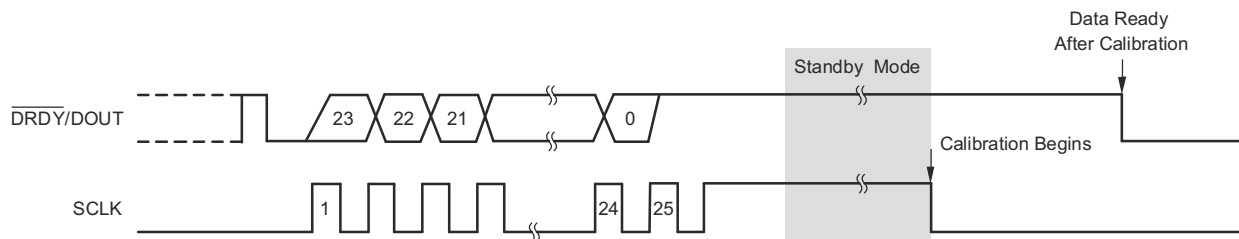
Figure 8-16. Summary of Serial Interface Waveforms
