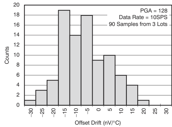
Figure 6-14. Offset Drift (25°C to 105°C)
