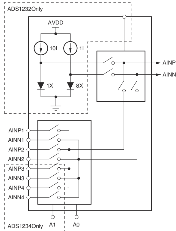
Figure 8-1. Measurement of the Temperature Sensor in the Input Multiplexer
