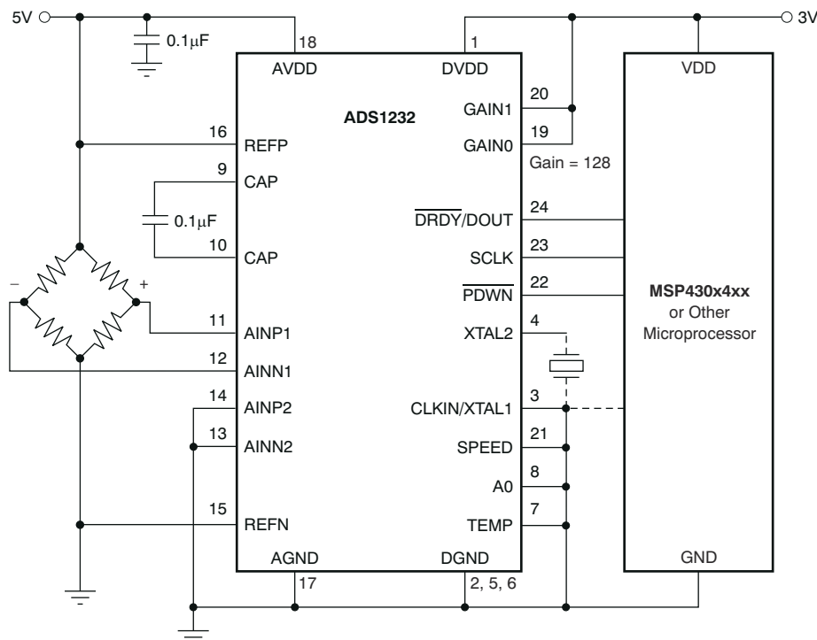
Figure 9-1. Weigh-Scale Application
