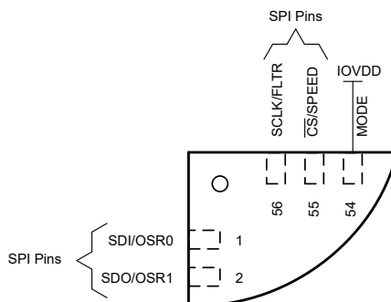
Figure 7-45. SPI Pins
