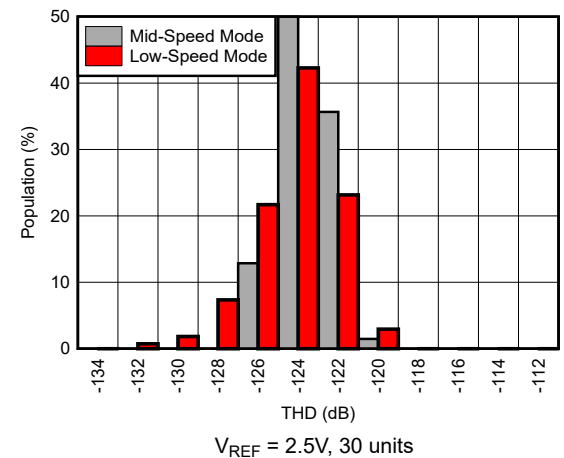
Figure 5-48. THD Histogram
