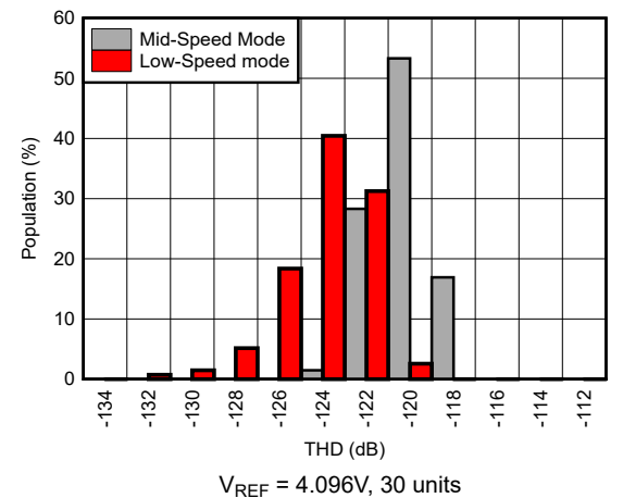
Figure 5-49. THD Histogram
