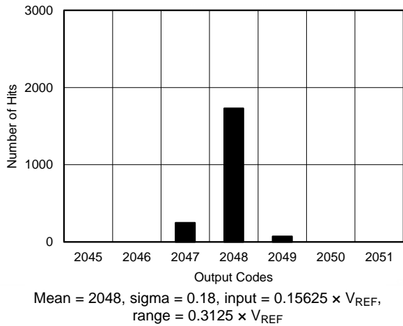
Figure 14. DC Histogram for Mid-Scale Inputs (0.3125 x V_{REF} )
