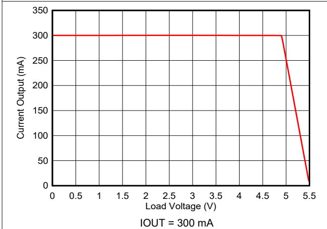
Figure 5-37. Current Output vs Load Voltage
