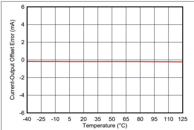
Figure 5-35. Current Output Offset Error vs Temperature
