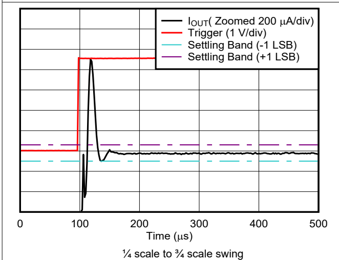
Figure 5-39. Current Output Setting Time, Rising Edge
