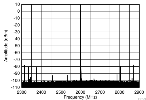
Figure 7-429. TX Single Tone (-6 dBFS) Output Spectrum at 2.6 GHz ( \pm 300 MHz)
