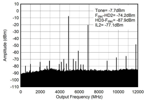
Figure 7-546. TX Single Tone (-1 dBFS) Output Spectrum at 4.9 GHz (0- f_{DAC} )
