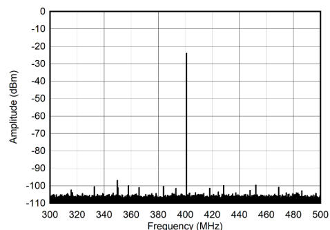
Figure 7-286. Single Tone Spectrum at 400 MHz and -30 dBFS (±100MHz)
