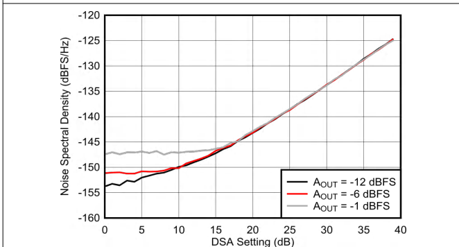
Figure 7-581. NSD vs DSA Setting and Amplitude at 7.1 GHz
