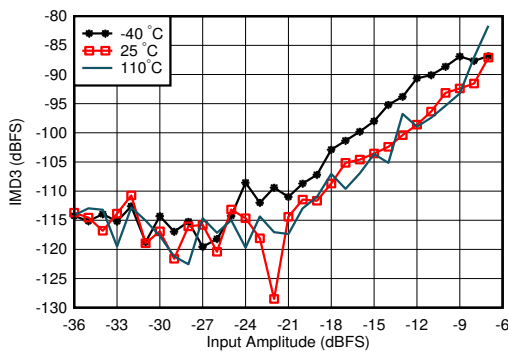
Figure 7-189. RX IMD3 vs Input Level and Temperature at 4.9 GHz
