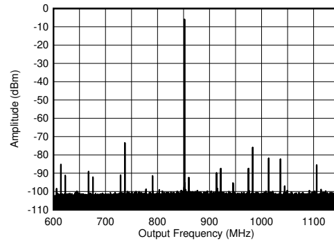
Figure 7-352. TX Single Tone (-12 dBFS) Output Spectrum at 0.85 GHz ( \pm 300 MHz)
