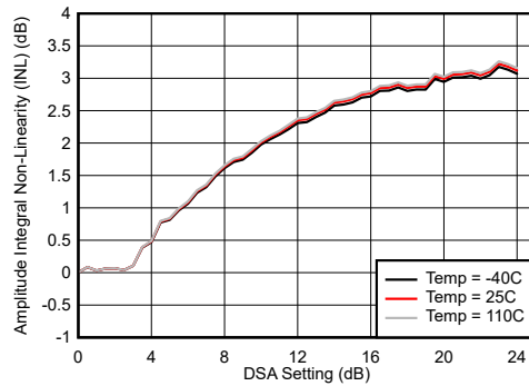
Integrated Amplitude Error = P_{\text{IN}}(\text{DSA Setting}) - P_{\text{IN}}(\text{DSA Setting} = 0) + (\text{DSA Setting}) Figure 7-4. RX Uncalibrated Integrated Amplitude Error vs DSA Setting at 30 MHz
