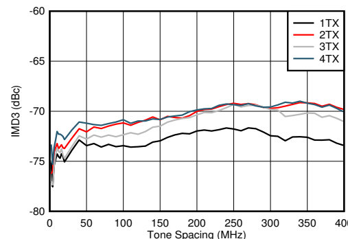
Figure 7-407. TX IMD3 vs Tone Spacing and Channel at 2.6 GHz
