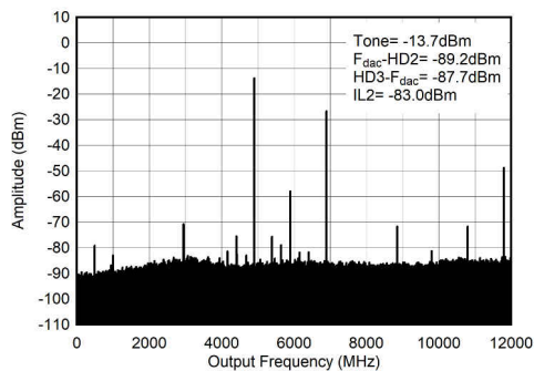
Figure 7-548. TX Single Tone (-6 dBFS) Output Spectrum at 4.9 GHz (0- f_{DAC} )
