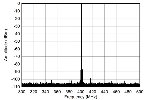
Figure 7-282. Single Tone Spectrum at 400 MHz and -6 dBFS (±100MHz)
