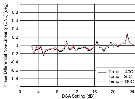
Differential Phase Error = \text{Phase}_{\text{IN}}(\text{DSA Setting} - 1) - \text{Phase}_{\text{IN}}(\text{DSA Setting}) Figure 7-6. RX Uncalibrated Differential Phase Error vs DSA Setting at 30 MHz
