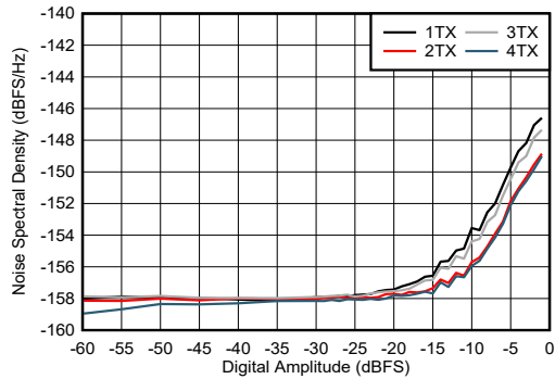
Figure 7-450. NSD vs Digital Amplitude and Channel at 2.6 GHz
