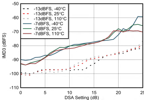
Figure 7-222. RX IMD3 vs DSA Setting at 6.851 GHz
