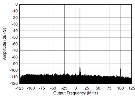
Figure 7-39. RX Output FFT at 405 MHz and -6 dBFS
