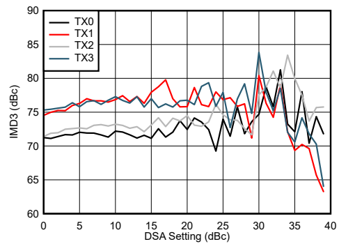
Figure 7-574. IMD3 vs DSA Setting and Channel at 7.1 GHz
