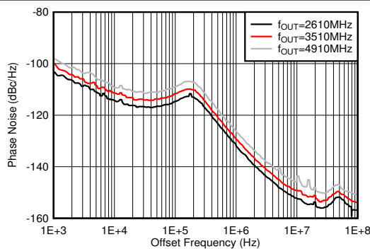
Figure 7-601. Phase Noise for 12-GHz VCO vs Offset Frequency and f_{\text{OUT}} at 25°C
