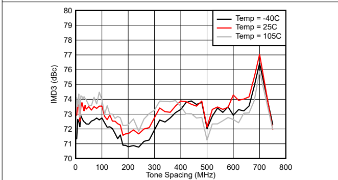
Figure 7-579. IMD3 vs Tone Spacing and Temperature at 7.1 GHz
