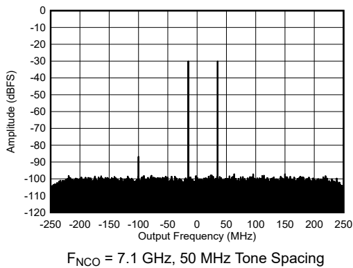
Figure 7-218. Dual Tone RX Output FFT at 7.1 GHz and -30 dBFS per Tone
