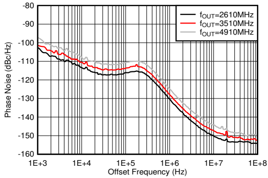
Figure 7-615. Phase Noise for 10-GHz VCO vs Offset Frequency and f_{OUT} at 110°C
