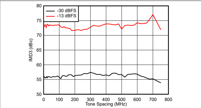
Figure 7-578. IMD3 vs Tone Spacing and Digital Amplitude at 7.1 GHz
