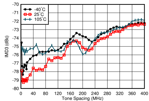
Figure 7-330. TX IMD3 vs Tone Spacing and Channel at 0.85 GHz
