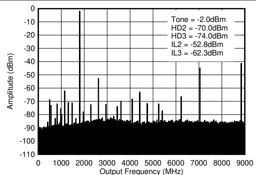
f_{\text{DAC}} = 8847.36 MSPS, interleave mode, 1.8 GHz matching, includes PCB and cable losses. \text{IL}_n = f_{\text{S}}/n \pm f_{\text{OUT}} . Figure 7-374. TX Single Tone (-6 dBFS) Output Spectrum at 1.8 GHz ( 0-f_{\text{DAC}} )
