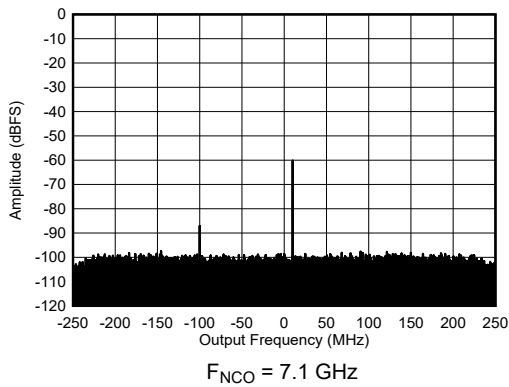
Figure 7-216. Single Tone RX Output FFT at 7.1 GHz and -60 dBFS
