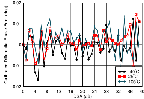
f_{\text{DAC}} = 5898.24 MSPS, interleave mode, matching at 0.8 GHz, channel with the median variation over DSA setting at 25°C Differential Phase Error = \text{Phase}_{\text{OUT}}(\text{DSA Setting} - 1) - \text{Phase}_{\text{OUT}}(\text{DSA Setting}) + 1
