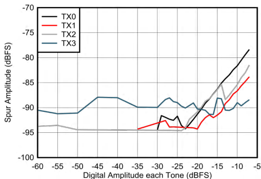
Inband = 2600 MHz \pm 600 MHz, f_{\text{DAC}} = 12 GSPS, not including F_s/3 and F_s/4 , external clock mode, non-interleave mode
