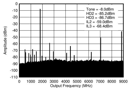
f_{\text{DAC}} = 8847.36 MSPS, interleave mode, 1.8 GHz matching, includes PCB and cable losses. \text{IL}_n = f_{\text{S}}/n \pm f_{\text{OUT}} . Figure 7-372. TX Single Tone (-12 dBFS) Output Spectrum at 1.8 GHz ( 0-f_{\text{DAC}} )
