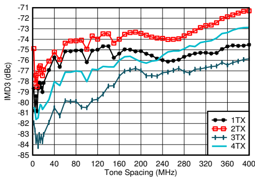
Figure 7-329. TX IMD3 vs Tone Spacing and Channel at 0.85 GHz
