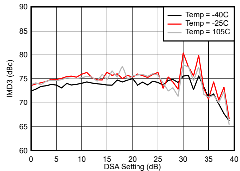
Figure 7-576. IMD3 vs DSA Setting and Temperature at 7.1 GHz
