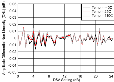
Differential Amplitude Error = P_{\text{IN}}(\text{DSA Setting} - 1) - P_{\text{IN}}(\text{DSA Setting}) + 1 Figure 7-3. RX Calibrated Differential Amplitude Error vs DSA Setting at 30 MHz
