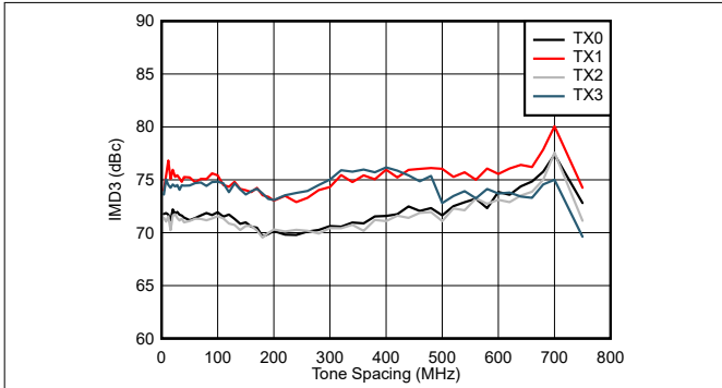
Figure 7-577. IMD3 vs Tone Spacing and Channel at 7.1 GHz
