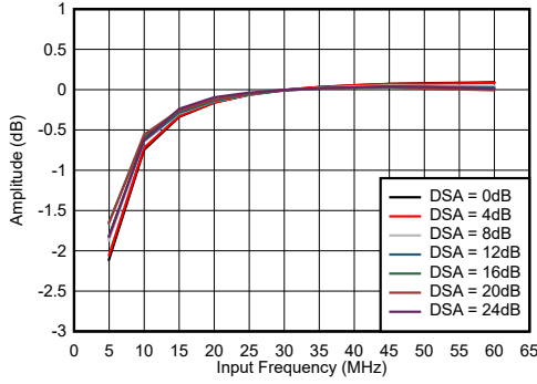
Normalized to 30 MHz Figure 7-1. RX In-Band Gain Flatness, f_{\text{IN}} = 30\text{ MHz}
