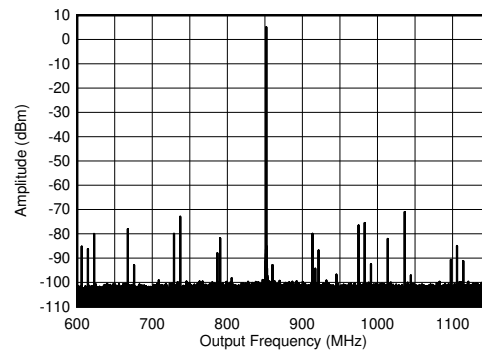
Figure 7-354. TX Single Tone (-6 dBFS) Output Spectrum at 0.85 GHz ( \pm 300 MHz)
