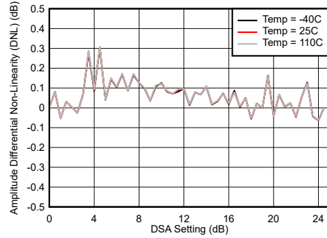
Differential Amplitude Error = P_{\text{IN}}(\text{DSA Setting} - 1) - P_{\text{IN}}(\text{DSA Setting}) + 1 Figure 7-2. RX Uncalibrated Differential Amplitude Error vs DSA Setting at 30 MHz
