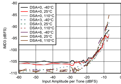
Figure 7-221. RX IMD3 vs Input Amplitude at 6.851 GHz
