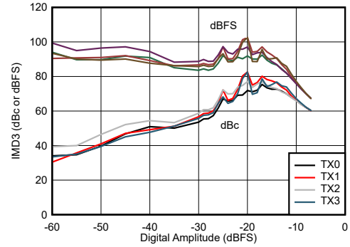
Figure 7-572. IMD3 vs Digital Amplitude and Channel at 7.1 GHz
