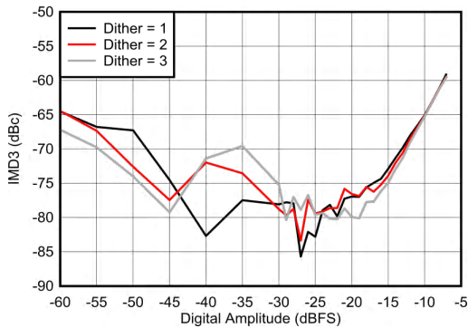
Figure 6-440. IMD3 vs Digital Amplitude and Dither at 2.6 GHz
