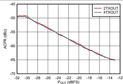
3.5 GHz Matching, single carrier 100-MHz BW NR TM1.1 Figure 6-481. TX 100-MHz NR ACPR vs Digital Level at 3.5 GHz
