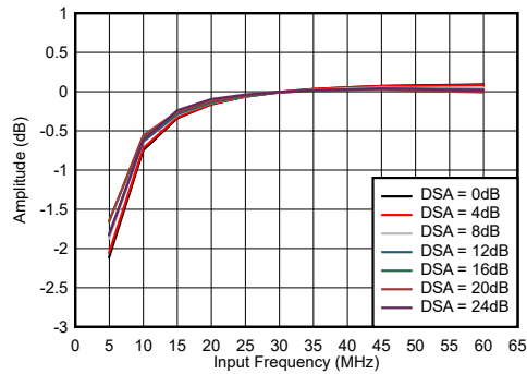
Normalized to 30 MHz Figure 6-1. RX In-Band Gain Flatness, f_{\text{IN}} = 30 MHz
