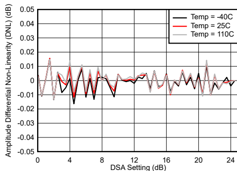
Differential Amplitude Error = P_{\text{IN}}(\text{DSA Setting} - 1) - P_{\text{IN}}(\text{DSA Setting}) + 1 Figure 6-3. RX Calibrated Differential Amplitude Error vs DSA Setting at 30 MHz
