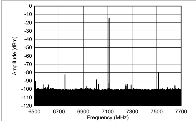
Figure 6-580. Single Tone Output Spectrum at 7.1 GHz, -6 dBFS (narrow span)
