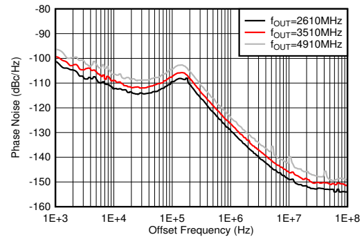
Figure 6-617. Phase Noise for 9-GHz VCO vs Offset Frequency and f_{OUT} at 25°C
