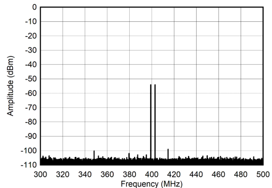
Figure 6-286. Dual Tone Spectrum at 400 MHz and -60 dBFS ( \pm 100 MHz)
