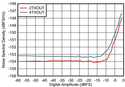
Figure 6-572. NSD vs DSA Setting and Amplitude at 7.1 GHz
