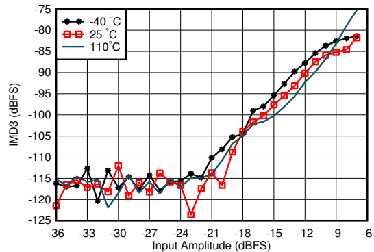
Figure 6-190. RX IMD3 vs Input Level and Temperature at 4.9 GHz
