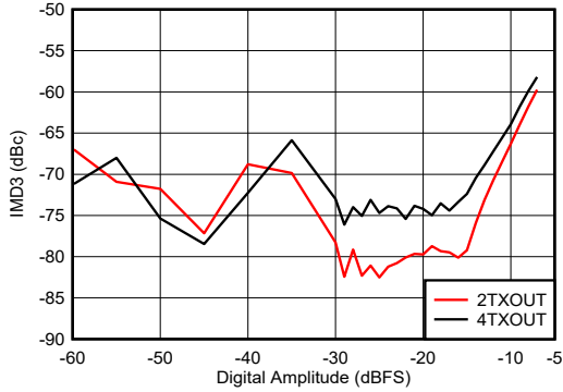
Figure 6-438. IMD3 vs Digital Amplitude and Channel at 2.6 GHz
