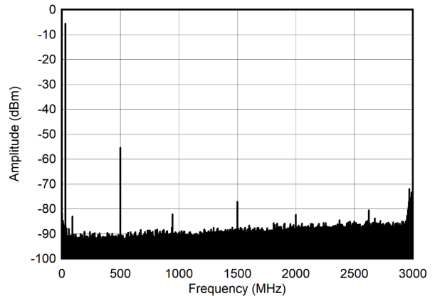
Figure 6-244. Single Tone Spectrum at 30 MHz and -12 dBFS (Nyquist)
