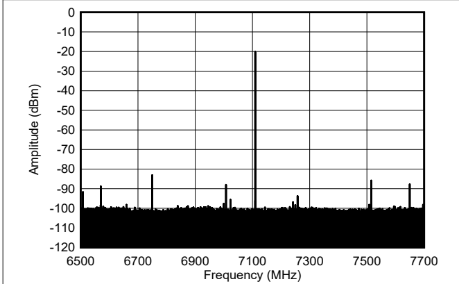
Figure 6-582. Single Tone Output Spectrum at 7.1 GHz, -12 dBFS (narrow span)
