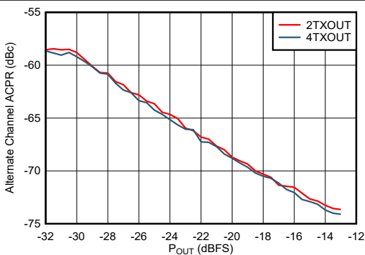
3.5 GHz Matching, single carrier 20-MHz BW TM1.1 LTE Figure 6-480. TX 20-MHz LTE alt-ACPR vs Digital Level at 3.5 GHz
