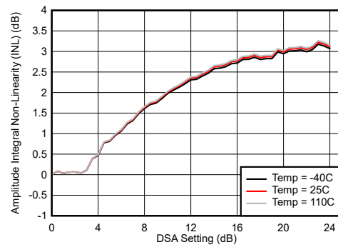
Integrated Amplitude Error = P_{\text{IN}}(\text{DSA Setting}) - P_{\text{IN}}(\text{DSA Setting} = 0) + (\text{DSA Setting}) Figure 6-4. RX Uncalibrated Integrated Amplitude Error vs DSA Setting at 30 MHz
