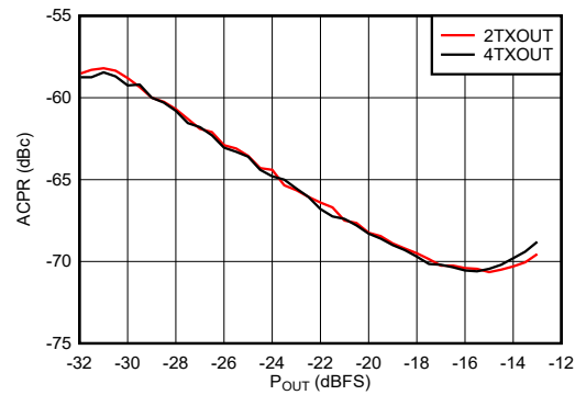
3.5 GHz Matching, single carrier 20-MHz BW TM1.1 LTE Figure 6-479. TX 20-MHz LTE ACPR vs Digital Level at 3.5 GHz
