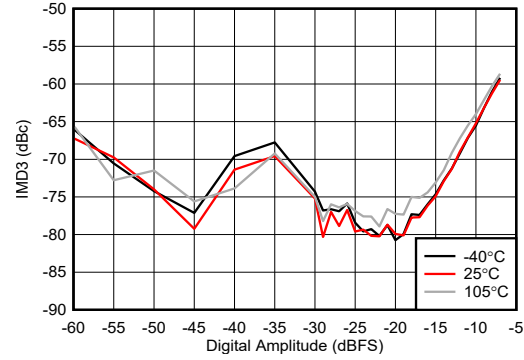
Figure 6-439. IMD3 vs Digital Amplitude and Temperature at 2.6 GHz
