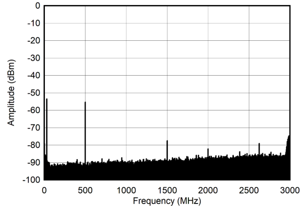
Figure 6-248. Single Tone Spectrum at 30 MHz and -60 dBFS (Nyquist)
