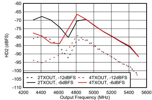
Matching at 4.9 GHz, f_{\text{DAC}} = 11.79648 GSPS, interleave mode, normalized to output power at harmonic frequency Figure 6-535. TX HD2 vs Digital Amplitude and Output Frequency at 4.9 GHz
