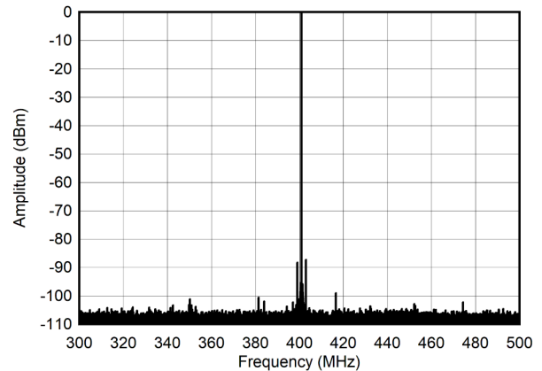
Figure 6-272. Single Tone Spectrum at 400 MHz and -6 dBFS ( \pm 100\text{MHz} )
