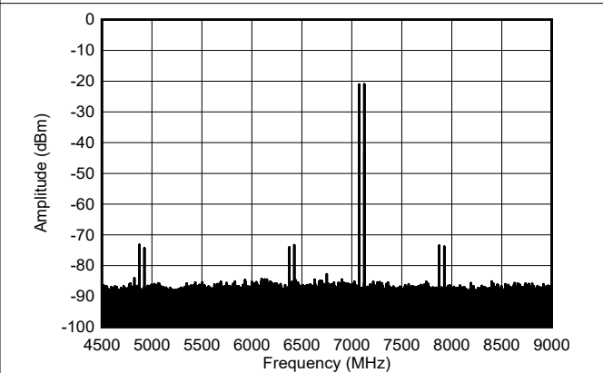
Figure 6-583. Two Tone Output Spectrum at 7.1 GHz, -7 dBFS each (Nyquist)
