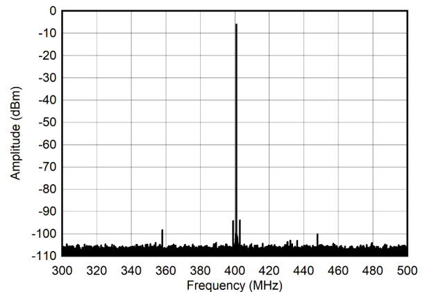
Figure 6-274. Single Tone Spectrum at 400 MHz and -12 dBFS ( \pm 100\text{MHz} )
