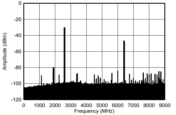
f_{\text{DAC}} = 9000 MSPS, external clock mode, non-interleave mode Figure 6-432. TX Dual Tone Output Spectrum at 2.6 GHz, -30 dBFS each (0 - DAC)
