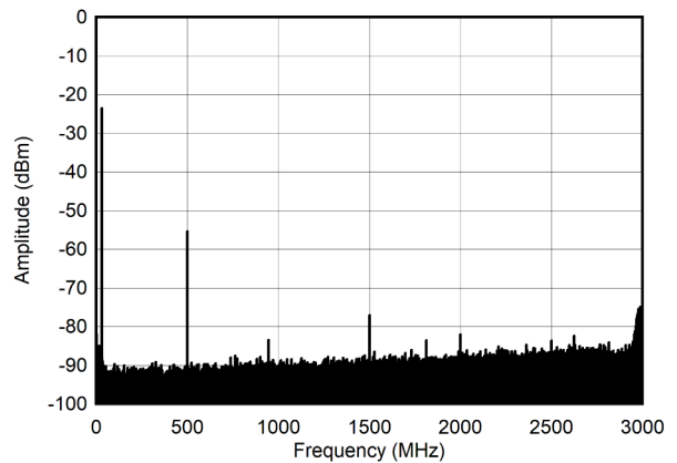
Figure 6-246. Single Tone Spectrum at 30 MHz and -30 dBFS (Nyquist)
