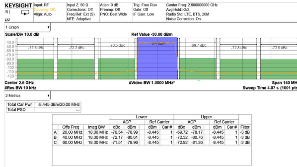
Figure 6-402. TX 20-MHz LTE Output Spectrum at 2.6 GHz (Band 41)
