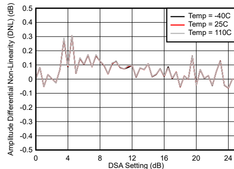
Differential Amplitude Error = P_{\text{IN}}(\text{DSA Setting} - 1) - P_{\text{IN}}(\text{DSA Setting}) + 1 Figure 6-2. RX Uncalibrated Differential Amplitude Error vs DSA Setting at 30 MHz
