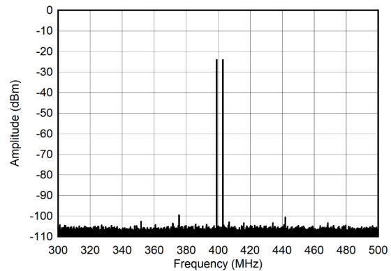
Figure 6-284. Dual Tone Spectrum at 400 MHz and -30 dBFS ( \pm 100 MHz)
