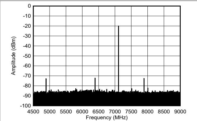
Figure 6-581. Single Tone Output Spectrum at 7.1 GHz, -12 dBFS (Nyquist)
