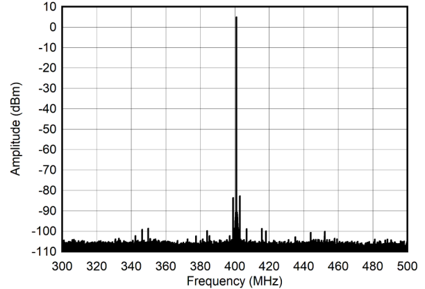
Figure 6-270. Single Tone Spectrum at 400 MHz and -1 dBFS ( \pm 100\text{MHz} )
