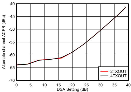
3.5 GHz Matching, single carrier 100-MHz BW NR TM1.1 Figure 6-478. TX 100-MHz NR alt-ACPR vs DSA Setting at 3.5 GHz
