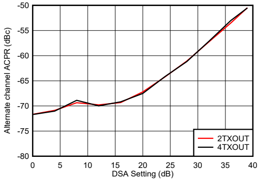
3.5 GHz Matching, single carrier 20-MHz BW TM1.1 LTE Figure 6-476. TX 20-MHz LTE alt-ACPR vs DSA Setting at 3.5 GHz
