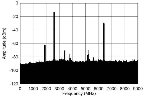
Figure 6-428. TX Dual Tone Output Spectrum at 2.6 GHz, -7 dBFS each ( 0 - DAC )
