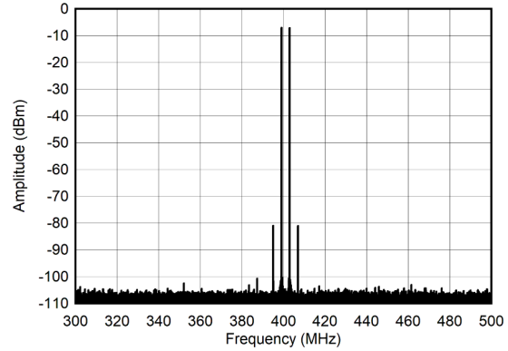
Figure 6-282. Dual Tone Spectrum at 400 MHz and -13 dBFS ( \pm 100 MHz)
