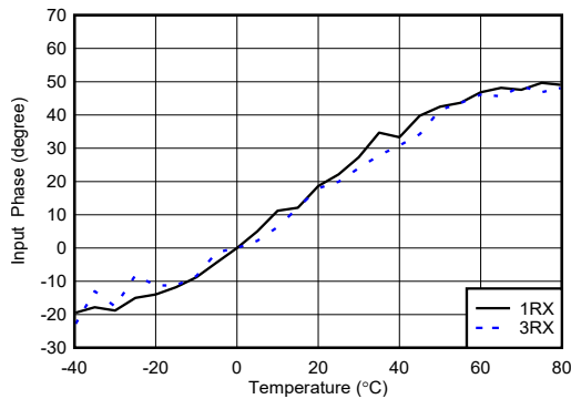
Figure 6-175. RX Input Phase vs Temperature and DSA at four = 4.9 GHz
