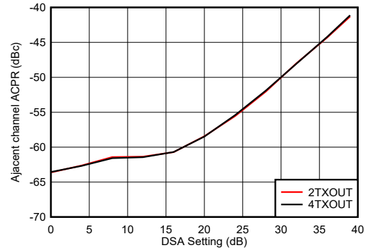
3.5 GHz Matching, single carrier 100-MHz BW NR TM1.1 Figure 6-477. TX 100-MHz NR ACPR vs DSA Setting at 3.5 GHz
