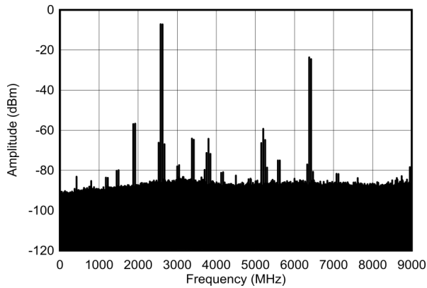
Figure 6-426. TX Single Tone (-1 dBFS) Output Spectrum at 2.6 GHz ( 0 - f_{DAC} )
