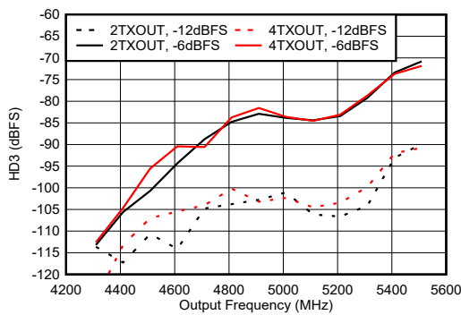
Matching at 4.9 GHz, f_{\text{DAC}} = 11.79648 GSPS, interleave mode, normalized to output power at harmonic frequency Figure 6-536. TX HD3 vs Digital Amplitude and Output Frequency at 4.9 GHz
