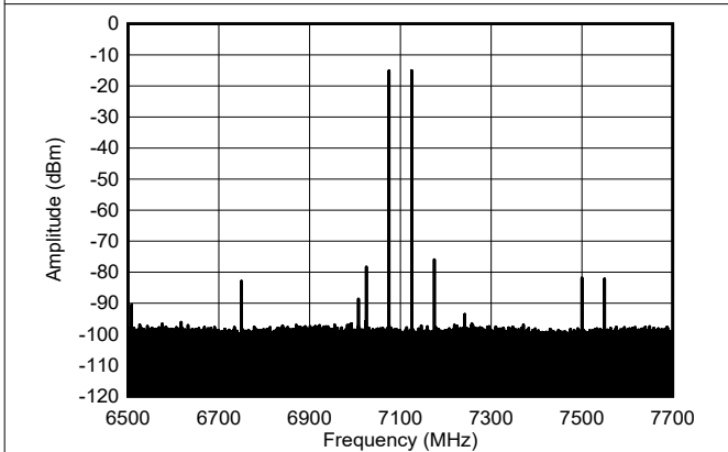
Figure 6-584. Two Tone Output Spectrum at 7.1 GHz, -7 dBFS each (narrow band)
