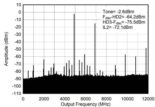
f_{\text{DAC}} = 11796.48 MSPS, interleave mode, 4.9 GHz matching, includes PCB and cable losses. IL_n = f_s/n \pm f_{\text{OUT}} . Figure 6-537. TX Single Tone (-1 dBFS) Output Spectrum at 4.9 GHz ( 0-f_{\text{DAC}} )
