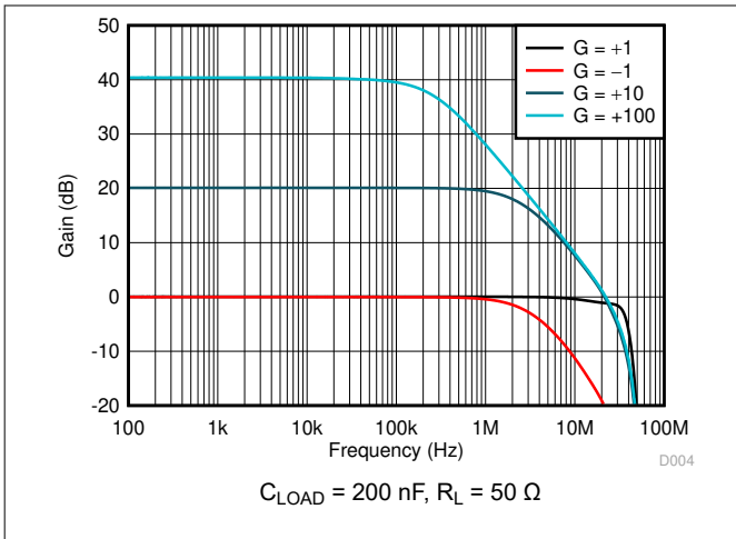
Figure 6-7. Closed-Loop Gain vs Frequency
