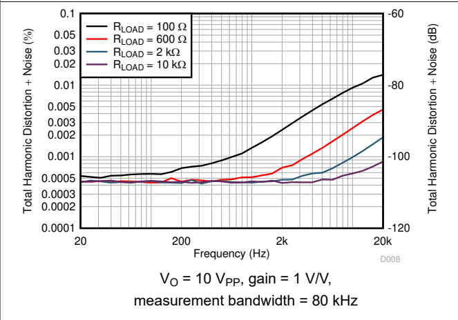
Figure 6-10. THD+N Ratio vs Frequency
