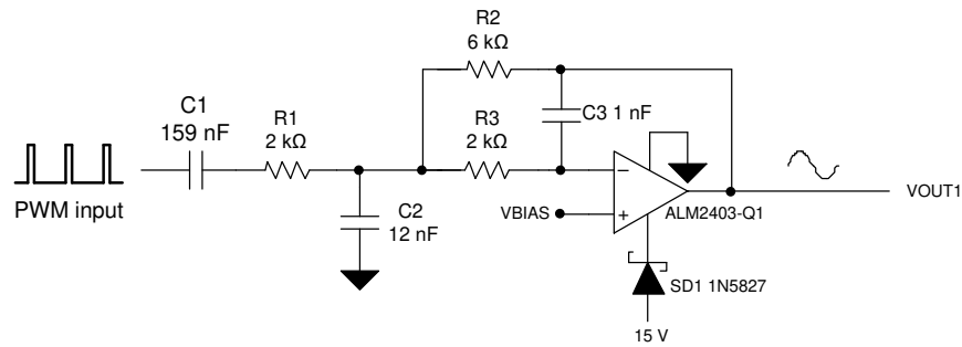
Figure 8-3. Two-Pole MFB Filter
