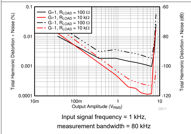
Figure 6-11. THD+N vs Output Amplitude
