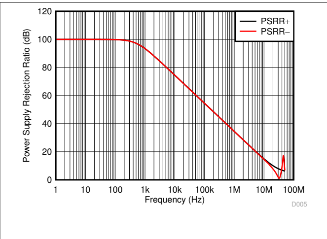
Figure 6-8. PSRR vs Frequency
