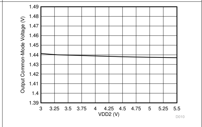
Figure 6-40. Output Common-Mode Voltage vs Low-Side Supply Voltage
