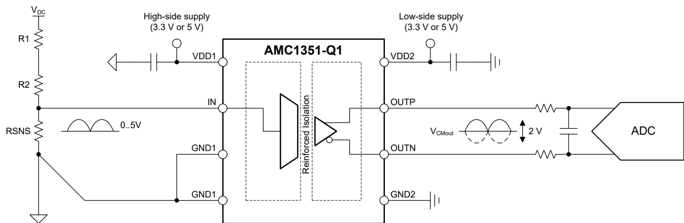
Typical Application
