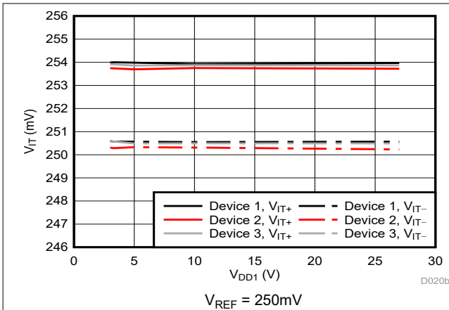
Figure 5-12. Cmp0 Trip Threshold vs Supply Voltage
