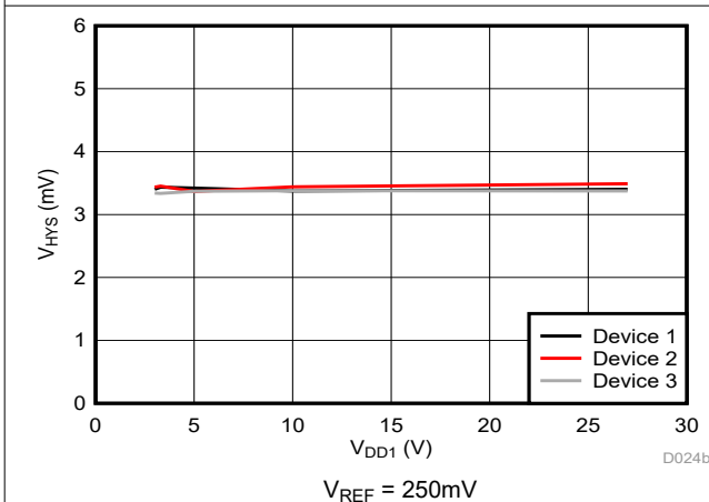
Figure 5-16. Cmp0 Trip Threshold Hysteresis vs Supply Voltage
