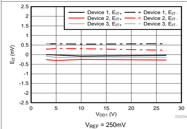
Figure 5-14. Cmp0 Trip Threshold Error vs Supply Voltage
