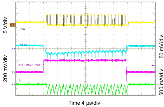
Figure 72. 1.2 V_{SYS} Load Transient, 0 to 200 mA
