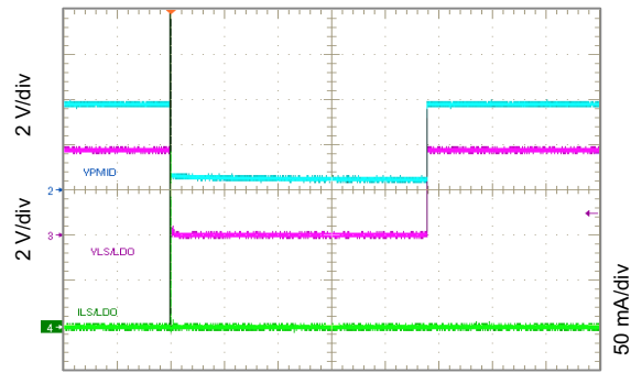
Figure 10-45. Short Circuit and Recovery for LS
