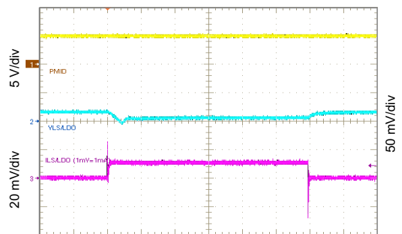
V_{LSLDO} = 1.2 \text{ V} Figure 10-48. 1.2 V LSLDO Load Transient, 0 to 10 mA
