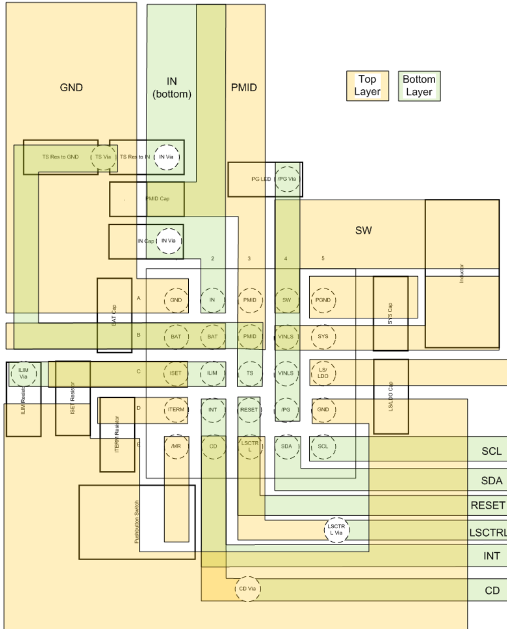
Figure 12-1. BQ25121A Layout
