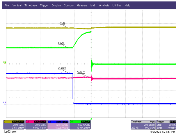
Figure 8-6. ISET Short-Circuit Response
