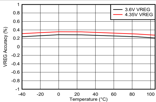
Figure 6-5. VSET Accuracy vs Temperature
