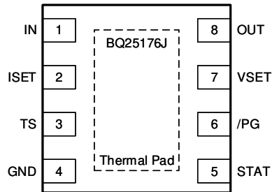
Figure 5-1. DSG Package 8-Pin WSON Top View
