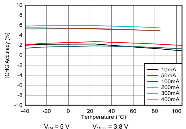
Figure 6-4. ICHG Accuracy vs Temperature
