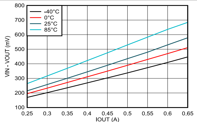
Figure 6-6. Dropout Voltage vs Output Current
