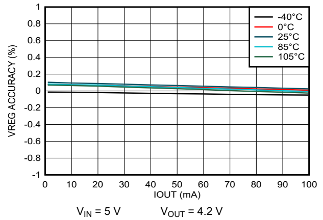
Figure 6-2. Load Regulation
