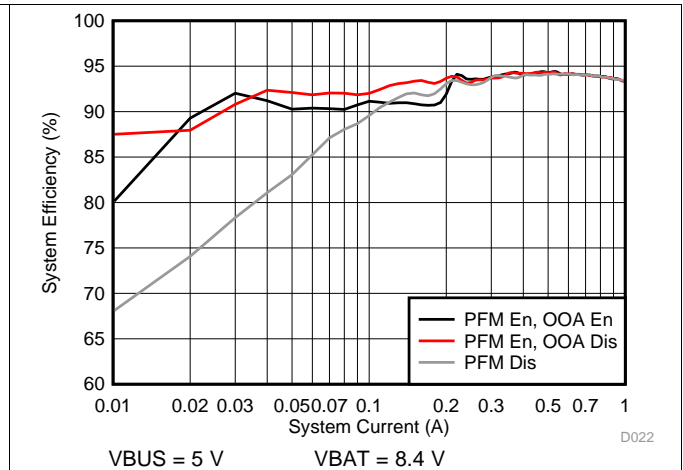
Figure 2. System Efficiency vs System Current
