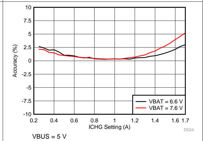
Figure 4. Charge Current Accuracy vs ICHG Setting
