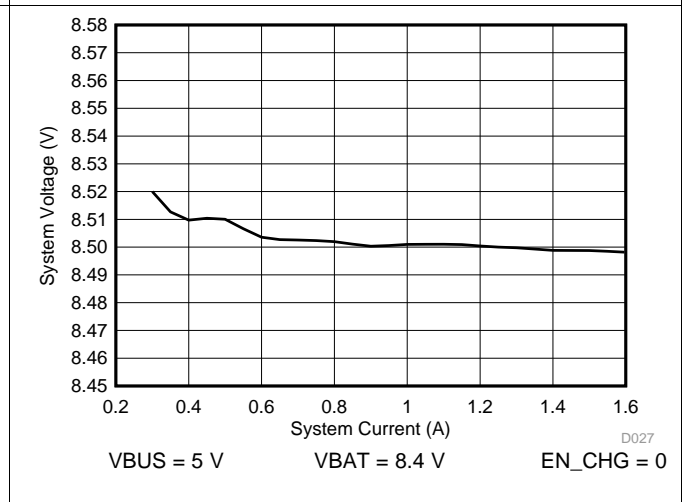
Figure 6. System Load Regulation After Charge Done
