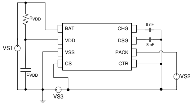
Figure 8-3. Test Circuit 3
