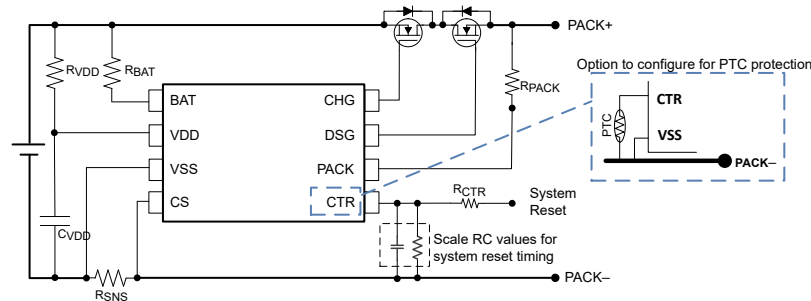
Simplified Schematic
