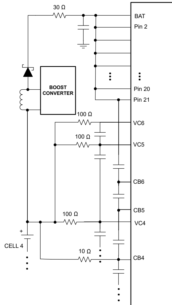
Figure 9-4. Unused VC and CB Channels - 4S
