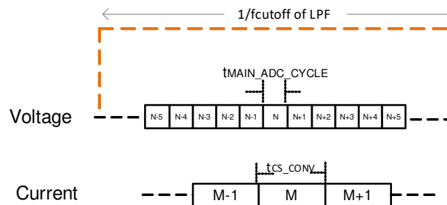
Figure 9-7. Effect of Voltage Low Pass Filter in Continuous Run Mode
