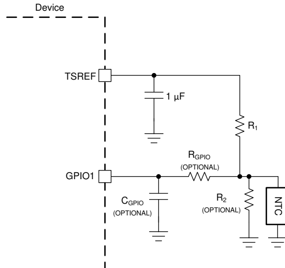
Figure 9-11. NTC Connection
