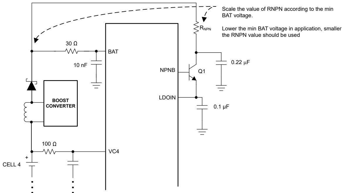
Figure 9-10. Boost Converter to Supply BAT in 4S Applications
