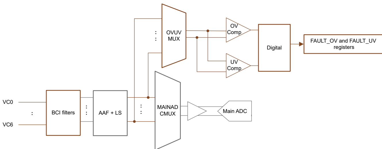
Figure 8-19. OV and UV Protectors
