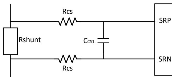
Figure 9-12. Current Sense Input Connection
