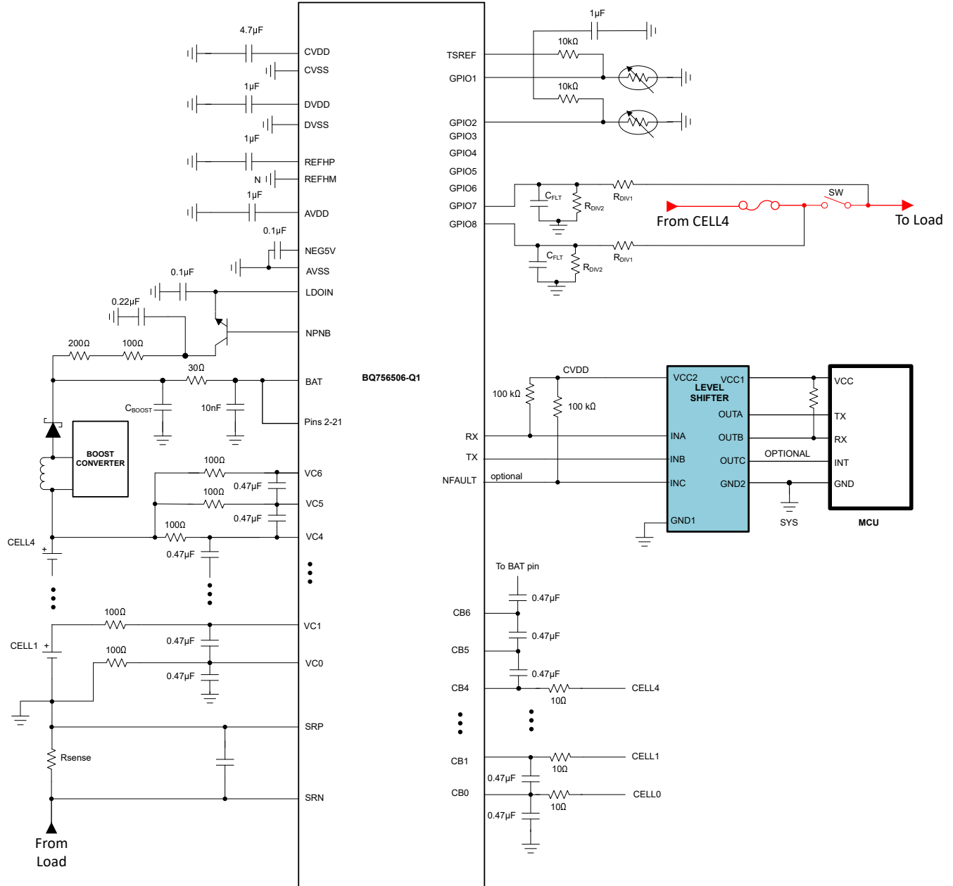
Figure 9-2. Typical Application Circuit - 4S
