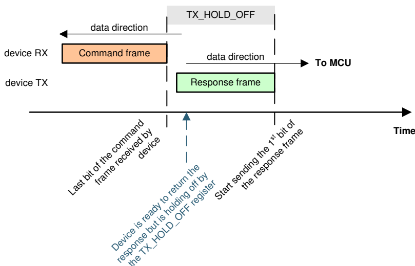
Figure 8-25. UART TX_HOLD_OFF
