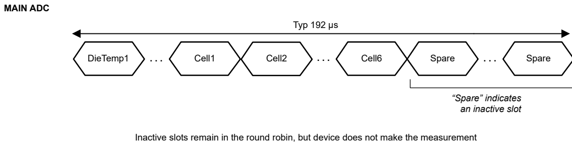
Figure 8-4. Same ADC Round Robin Timing for all Channel Counts
