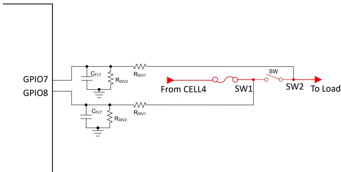
Figure 9-5. Fuse and Relay Status Detection
