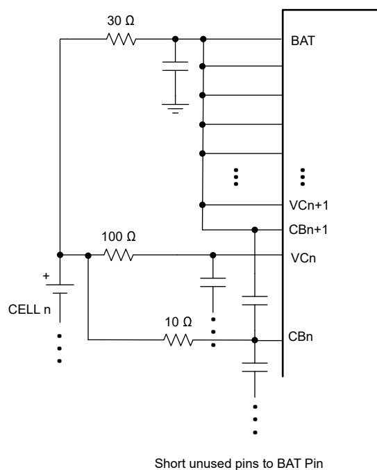
Figure 9-3. Unused VC and CB Channels - 6S
