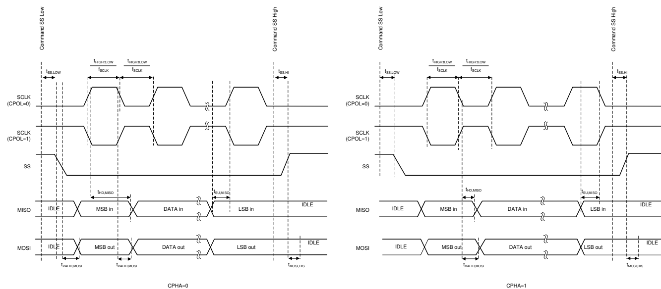
Figure 8-29. SPI Controller Timing Diagram
