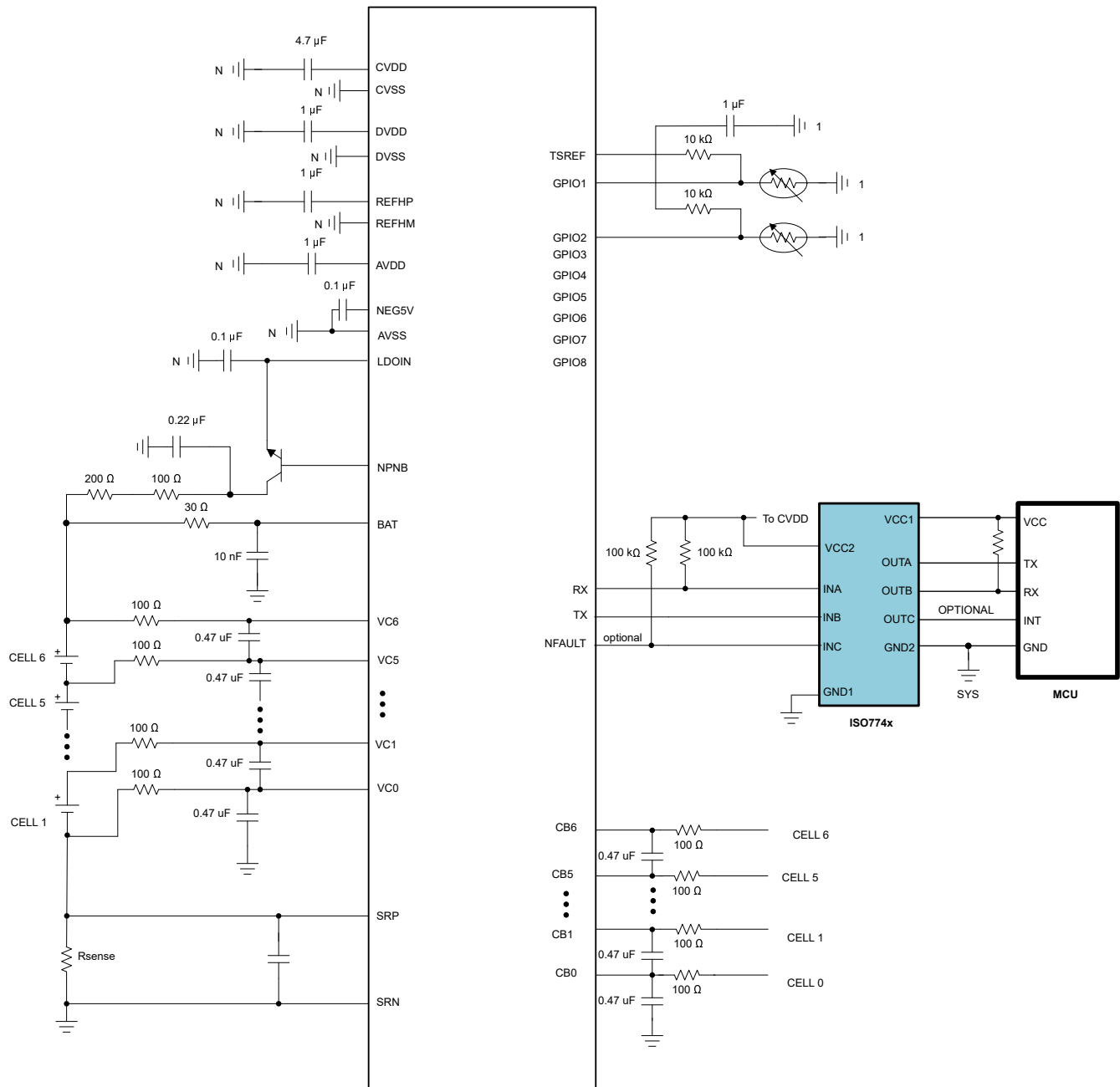
Figure 9-1. Typical Application Circuit - 6S
