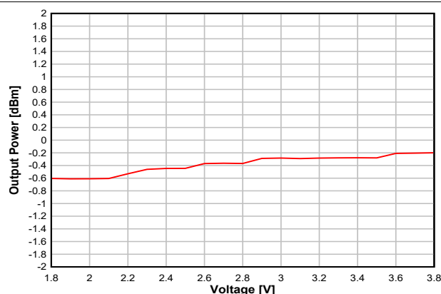
Figure 7-25. Output Power vs. Supply Voltage (VDD) (BLE 1 Mbps, 2.44GHz, 0dBm)
