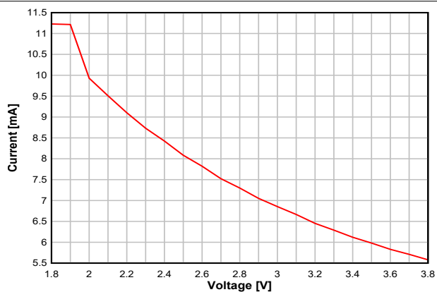
Figure 7-7. RX Current vs. Supply Voltage (VDDS) (BLE 1Mbps, 2.44GHz)
