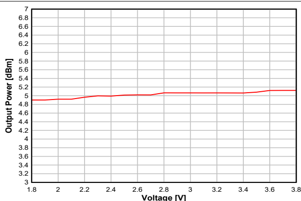
Figure 7-26. Output Power vs. Supply Voltage (VDD) (BLE 1 Mbps, 2.44GHz, +5dBm)
