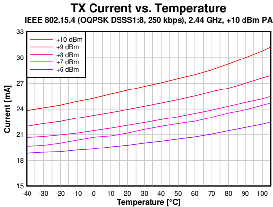
Figure 7-10. TX Current vs. Temperature (250kbps, 2.44GHz, +10dBm PA)
