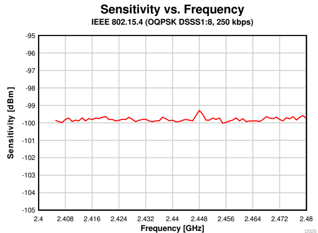
Figure 7-15. Sensitivity vs. Frequency (250 kbps, 2.44 GHz)
