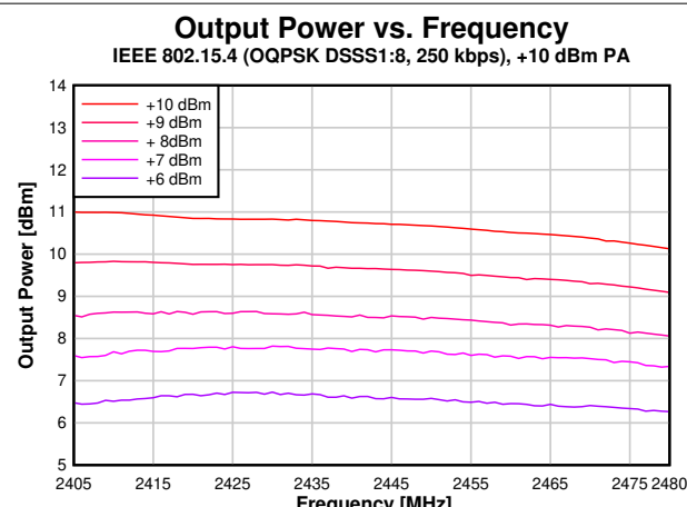
Figure 7-32. Output Power vs. Frequency (250 kbps, +10 dBm PA)
