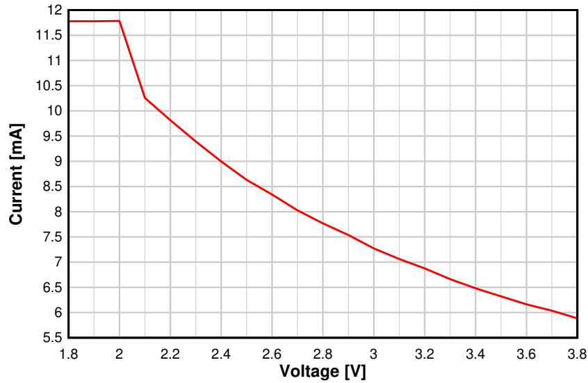
Figure 8-8. RX Current vs. Supply Voltage (VDD5) (BLE 1 Mbps, 2.44 GHz)
