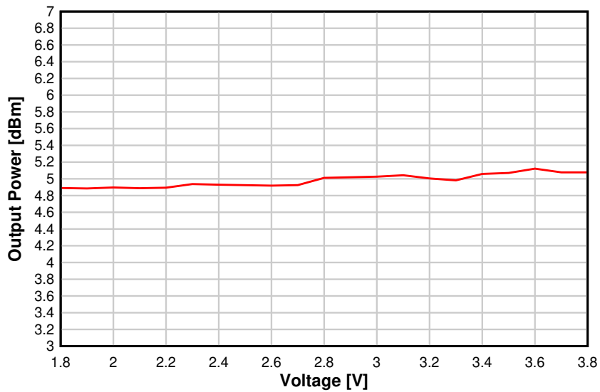
Figure 8-21. Output Power vs. Supply Voltage (VDD5) (BLE 1 Mbps, 2.44 GHz, +5 dBm)
