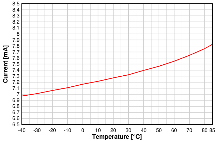
Figure 8-7. RX Current vs. Temperature (BLE 1 Mbps, 2.44 GHz)
