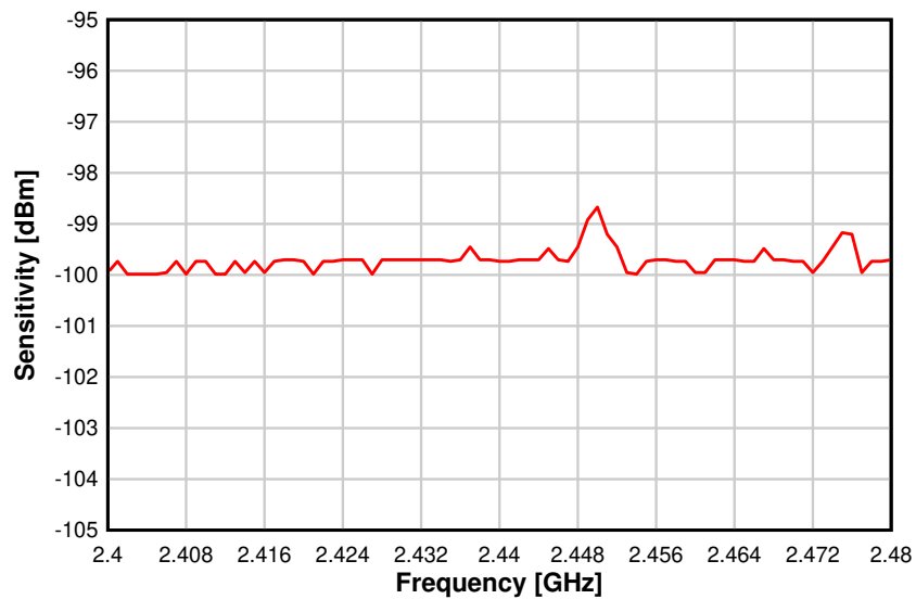
Figure 8-12. Sensitivity vs. Frequency IEEE 802.15.4 (OQPSK DSSS1:8, 250 kbps)
