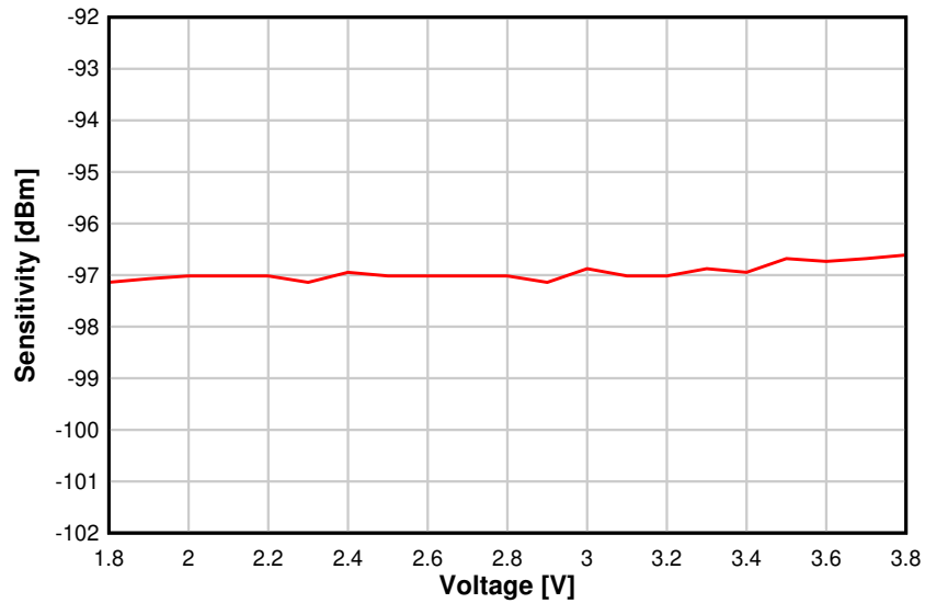
Figure 8-15. Sensitivity vs. Supply Voltage (VDDS) (BLE 1 Mbps, 2.44 GHz)
