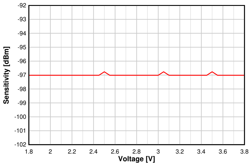
Figure 8-16. Sensitivity vs. Supply Voltage (VDDS) (BLE 1 Mbps, 2.44 GHz, DCDC Off)
