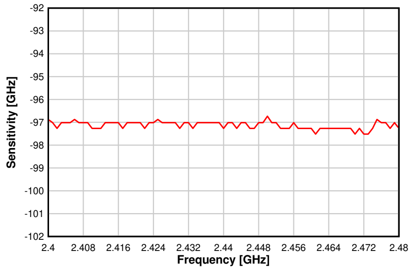
Figure 8-11. Sensitivity vs. Frequency (BLE 1 Mbps, 2.44 GHz)
