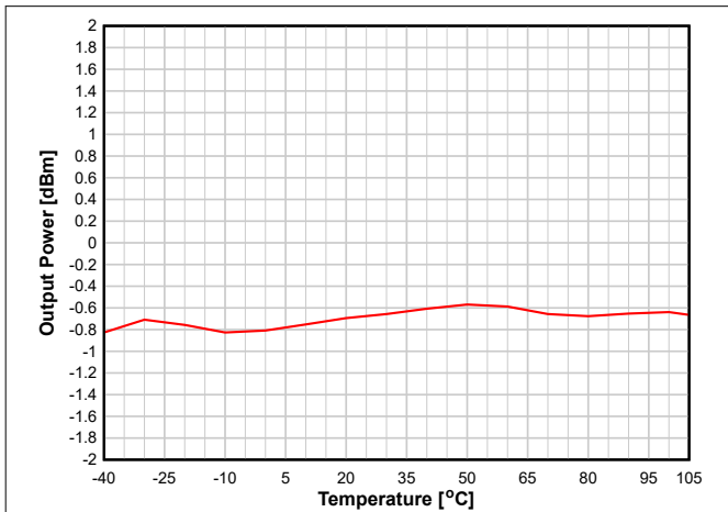
Figure 8-19. Output Power vs. Temperature (BLE 1 Mbps, 2.44 GHz, 0 dBm)
