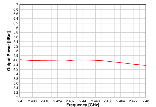
Figure 8-24. Output Power vs. Frequency (BLE 1 Mbps, +5 dBm)
