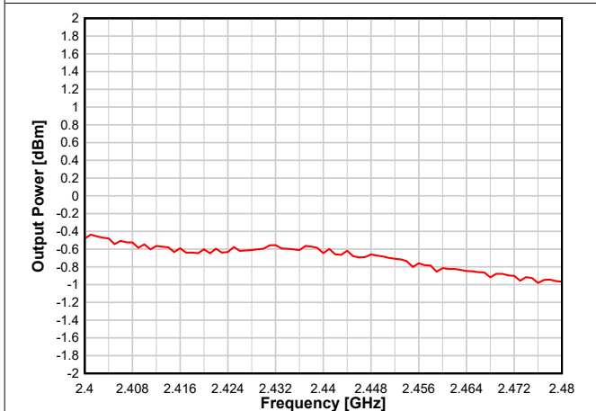
Figure 8-23. Output Power vs. Frequency (BLE 1 Mbps, 0 dBm)
