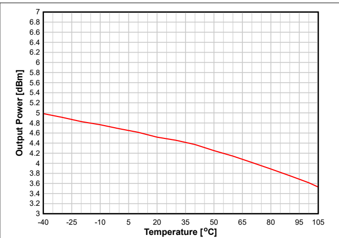
Figure 8-20. Output Power vs. Temperature (BLE 1 Mbps, 2.44 GHz, +5 dBm)
