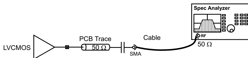
Figure 22. CDCUN1208LP LVCMOS Output – Phase Noise/Jitter Measurement Setup
