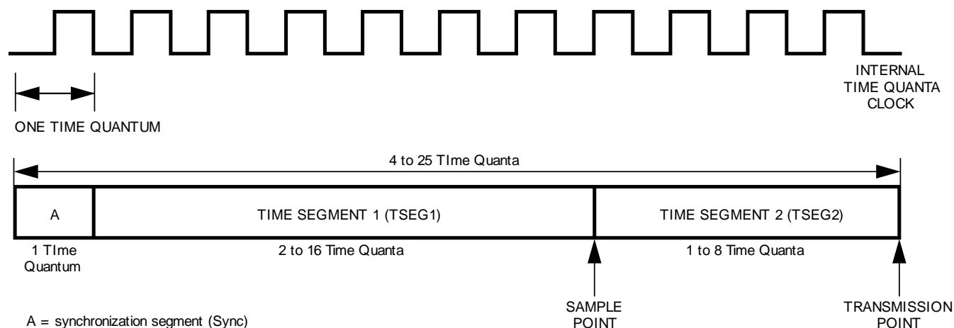
Figure 22-11. Bit Timing
