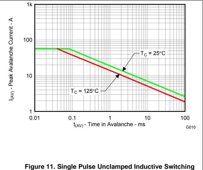
Figure 11. Single Pulse Unclamped Inductive Switching
