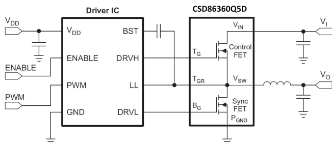
Typical Circuit
