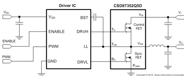
Typical Circuit
