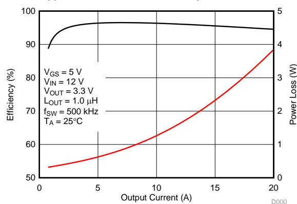
Typical Power Block Efficiency and Power Loss
