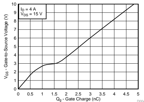
Gate Charge
