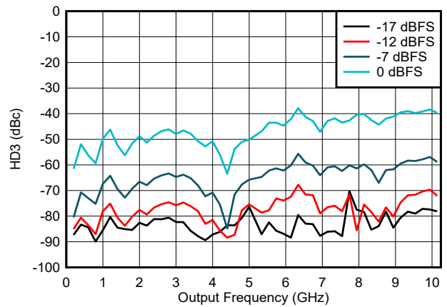
Figure 6-162. HD3 vs Frequency and Digital Amplitude in NRZ/RF Modes
