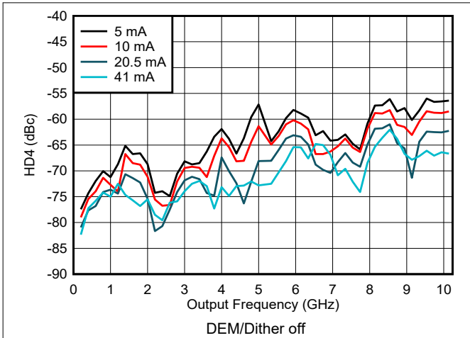
Figure 6-173. HD4 vs Frequency and Output Current in NRZ/RF Modes
