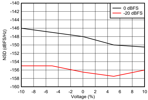
Figure 6-88. NSD vs Supply Voltage
