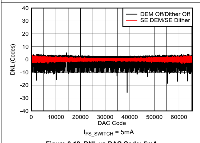
Figure 6-12. DNL vs DAC Code: 5mA
