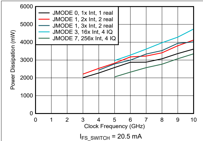
Figure 6-211. Power Dissipation vs Clock Frequency and Digital Mode
