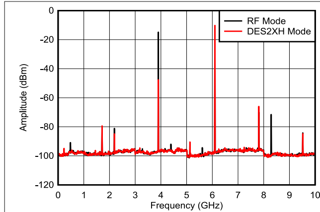
Figure 6-31. f_{\text{OUT}} = 6097\text{ MHz} , 0 dBFS
