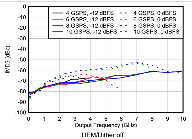
Figure 6-132. IMD3 vs Frequency and Sample Rate in DES2X Modes
