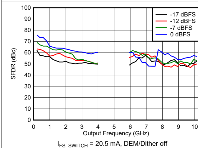
Figure 6-105. SFDR vs Frequency and Digital Amplitude in DES2X Modes
