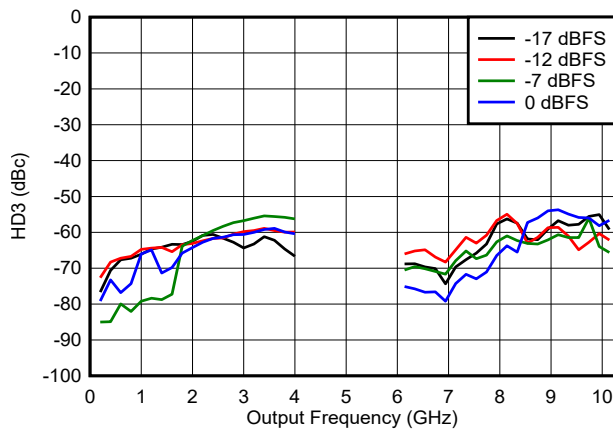
Figure 6-163. HD3 vs Frequency and Digital Amplitude in NRZ/RF Modes
