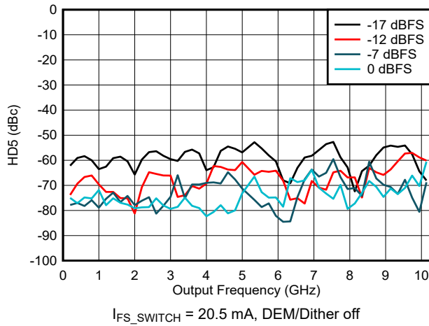
Figure 6-181. HD5 vs Frequency and Digital Amplitude in NRZ/RF Modes
