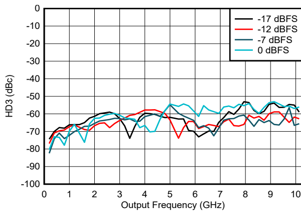
Figure 6-161. HD3 vs Frequency and Digital Amplitude in NRZ/RF Modes
