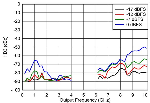
Figure 6-164. HD3 vs Frequency and Digital Amplitude in NRZ/RF Modes
