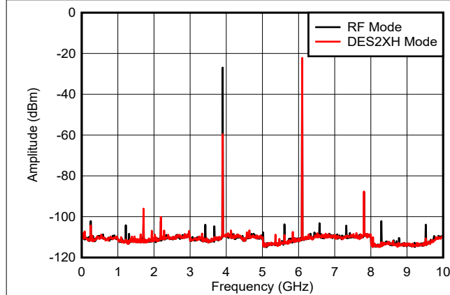
Figure 6-31. f_{\text{OUT}} = 6097\text{ MHz} , 0 dBFS
