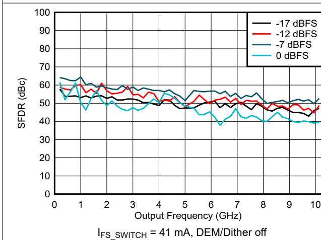
Figure 6-103. SFDR vs Frequency and Digital Amplitude in NRZ/RF Modes
