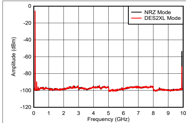
includes PCB, cable and balun loss Figure 6-19. f_{\text{OUT}} = 97\text{ MHz} , 0 dBFS
