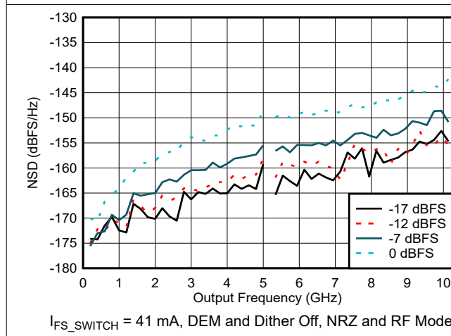
Figure 6-66. NSD vs Output Frequency and Digital Amplitude
