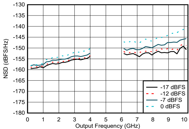
I_{FS\_SWITCH} = 41 mA, DEM and Dither On, DEM\_ADJ = 0 , DES2XL and DES2XH Modes
