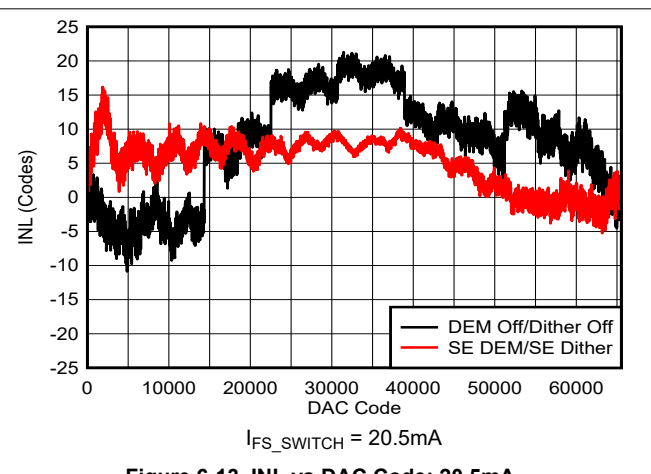
Figure 6-13. INL vs DAC Code: 20.5mA
