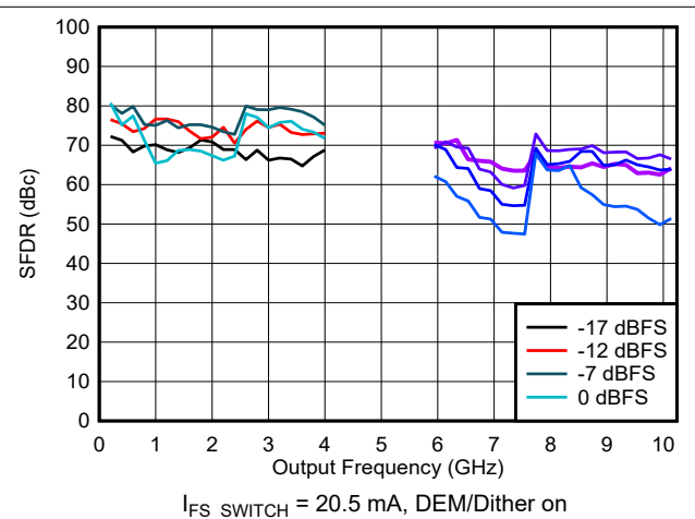
Figure 6-106. SFDR vs Frequency and Digital Amplitude in DES2X Modes
