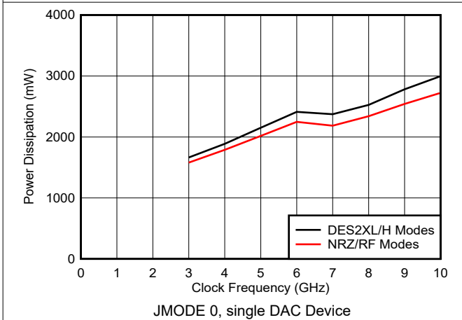
Figure 6-213. Power Dissipation vs Clock Frequency and DAC Mode
