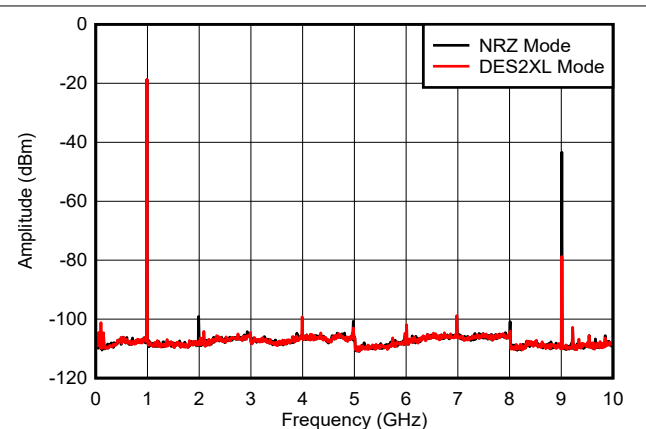
includes PCB, cable and balun loss Figure 6-22. f_{\text{OUT}} = 997\text{ MHz} , 0 dBFS
