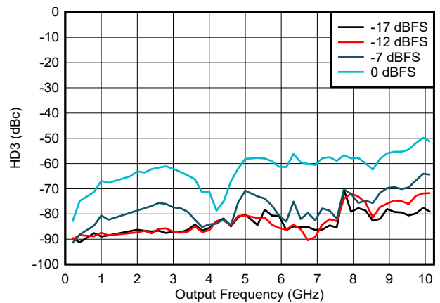
Figure 6-162. HD3 vs Frequency and Digital Amplitude in NRZ/RF Modes
