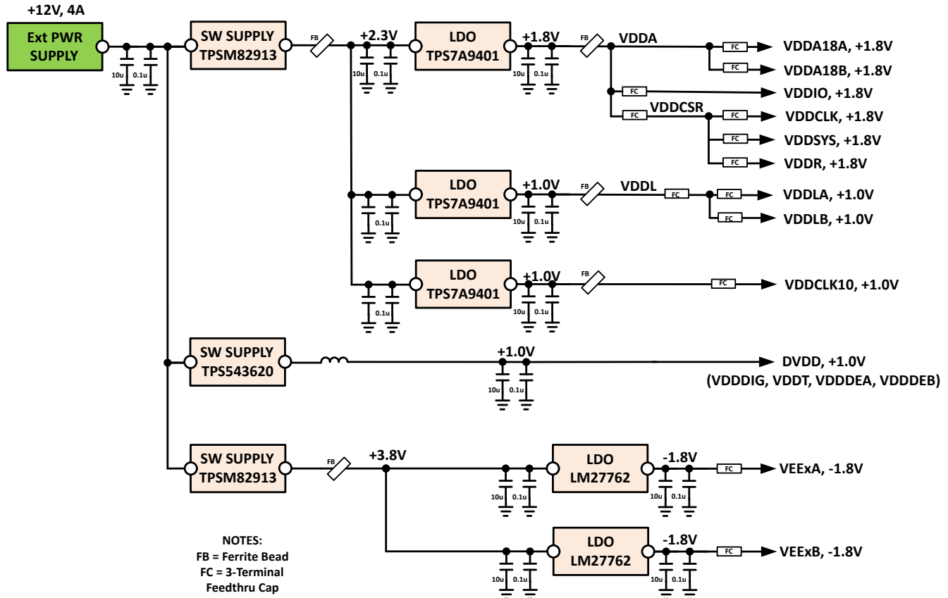
Figure 8-23. Recommended Power Supply Block Diagram
