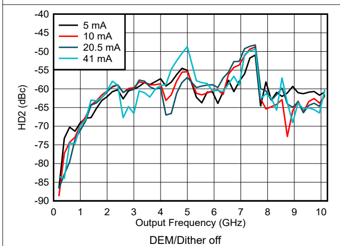
Figure 6-141. HD2 vs Frequency and Output Current in NRZ/RF Modes
