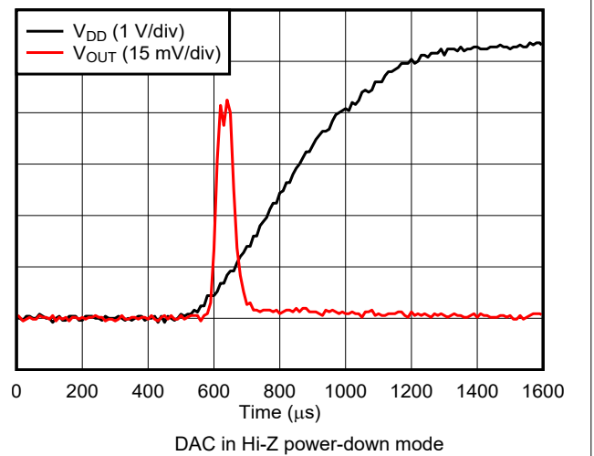
Figure 5-23. Voltage Output Power-On Glitch
