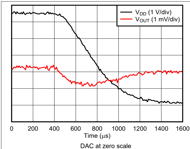
Figure 5-24. Voltage Output Power-Off Glitch
