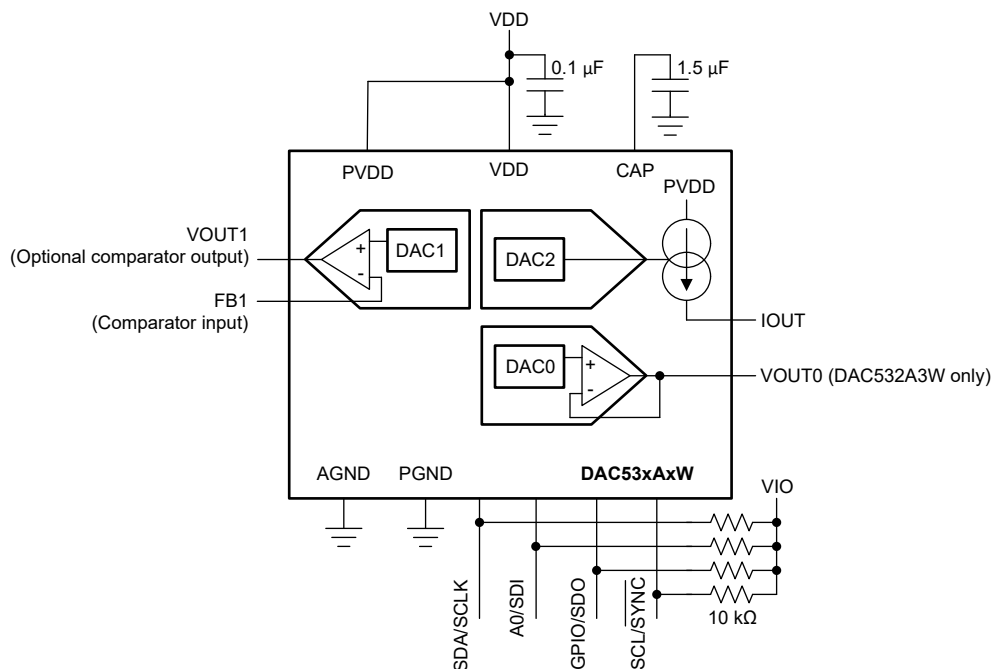
Figure 6-2. Comparator Interface
