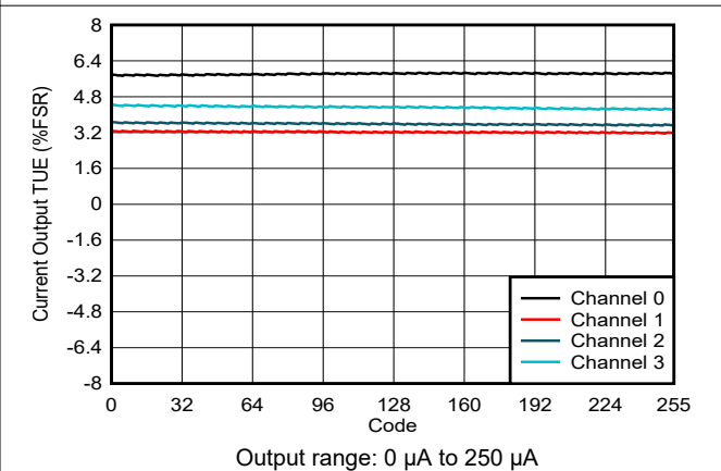
Figure 6-42. Current Output TUE vs Digital Input Code
