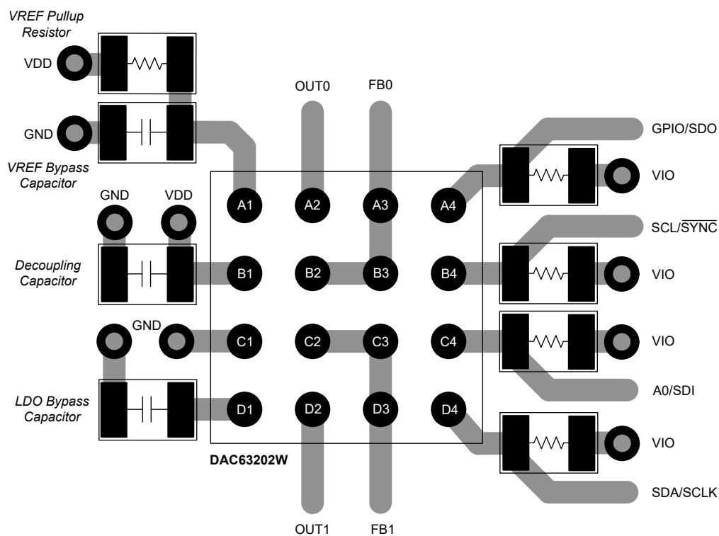
Figure 8-4. Layout Example
