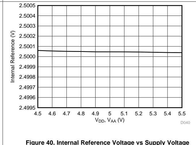
Figure 40. Internal Reference Voltage vs Supply Voltage
