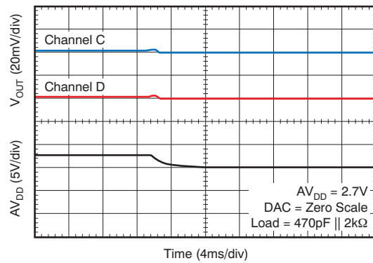
Figure 113. Power-Off Glitch
