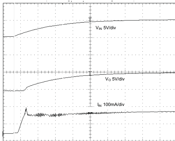
Figure 24. StartUp Waveforms
