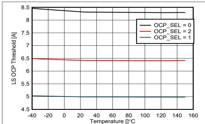
Figure 6-14. LS OCP Threshold vs Temperature at V_{VM} = 13.5\text{ V}
