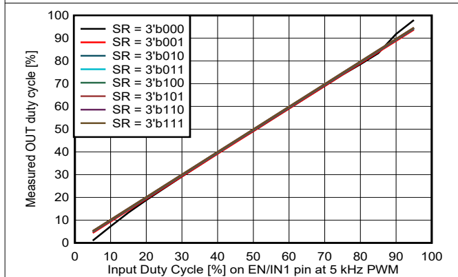
Figure 6-18. Measured Duty Cycle vs Input Duty Cycle at PWM frequency of 5 KHz at V_{VM} = 13.5\text{ V} for HS recirculation
