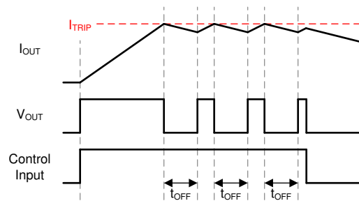
Figure 6-6. Current Regulation
