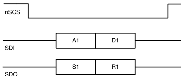
Figure 7-48. SPI Format - Standard "16-bit" Frame
