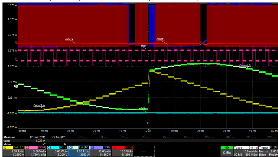
Figure 7-5. Indexer reset
