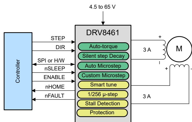
Simplified Schematic
