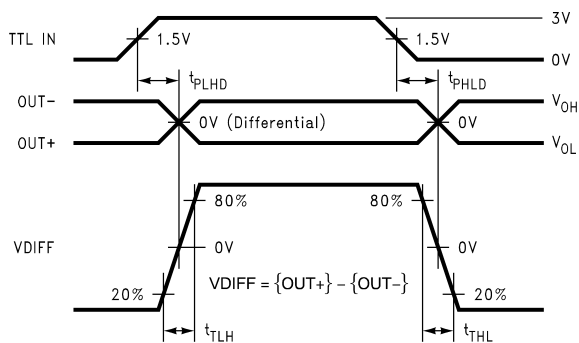
Figure 10. Differential Driver Propagation Delay and Transition Time Waveforms
