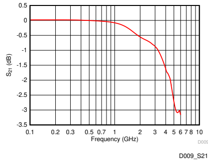
Figure 8-2. Insertion Loss Vs. Frequency
