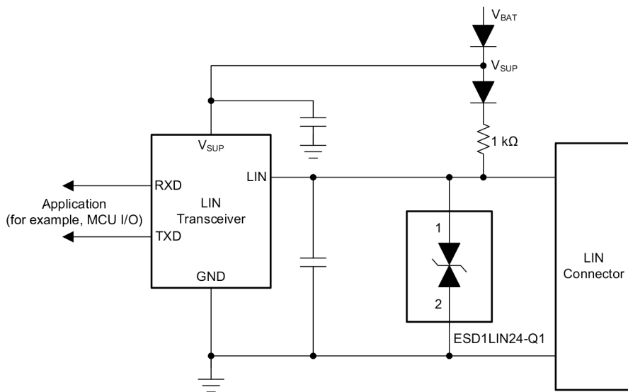
Typical Application
