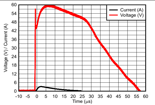
Figure 5-4. 8/20 μs Surge Response
