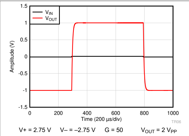
Figure 6-50. Large Signal Step Response
