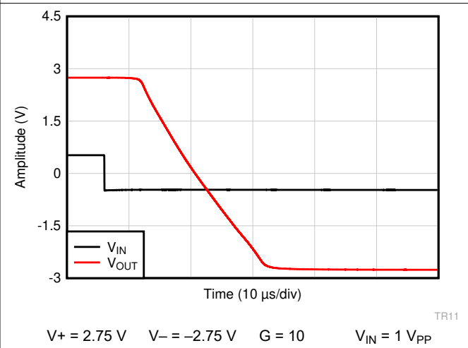
Figure 6-54. Over-Load Recovery (Falling Edge)
