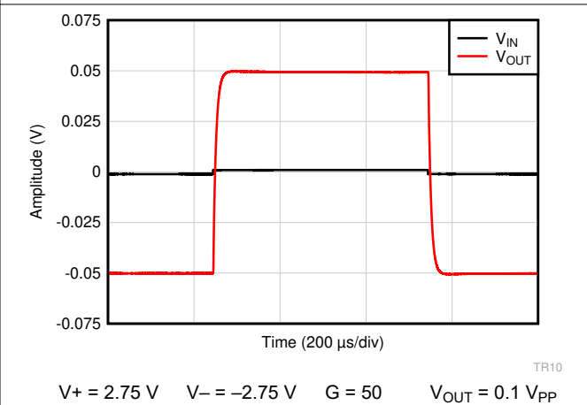
Figure 6-52. Small-Signal Step Response
