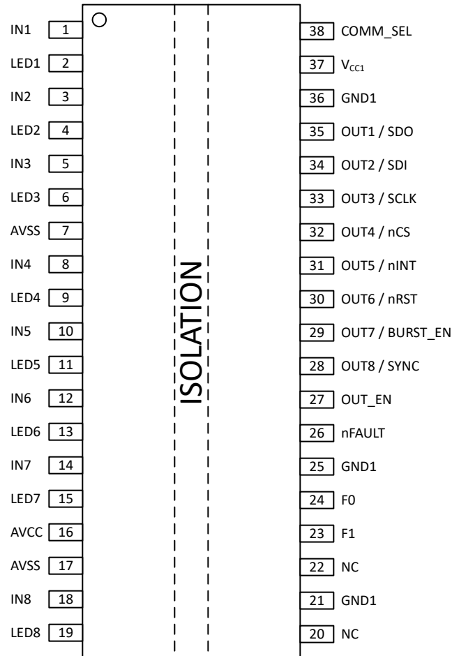
Figure 4-1. ISO1228
