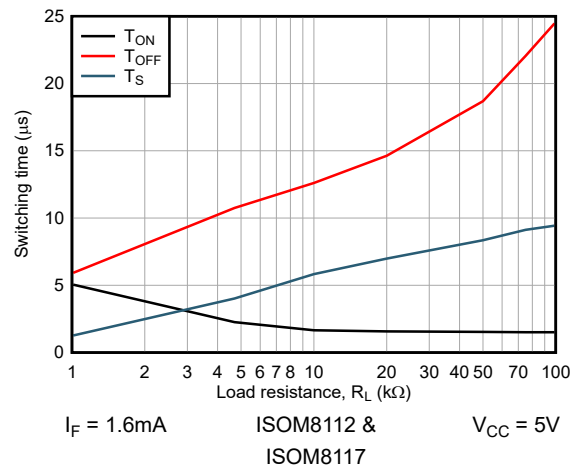
Figure 6-24. Switching Time vs Load Resistance
