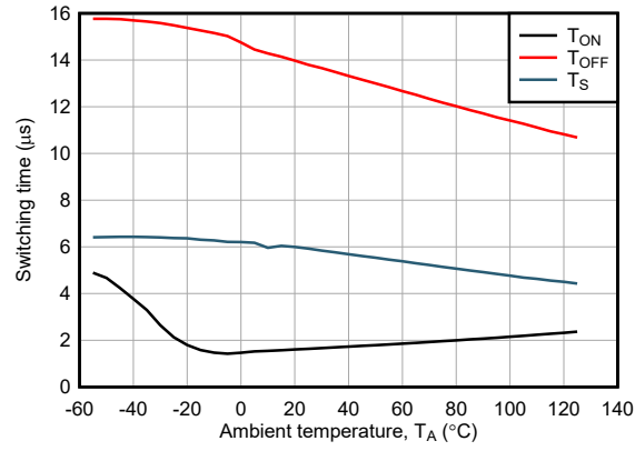
Figure 6-29. Switching Time vs Ambient Temperature
