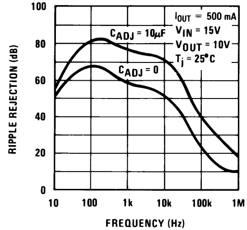
Figure 7-8. Ripple Rejection
