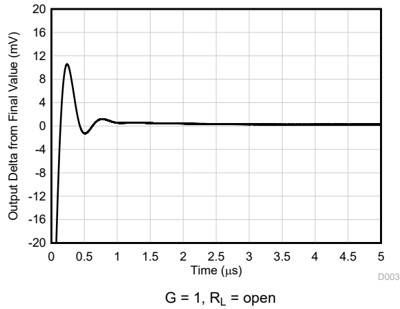
Figure 5-31. Large-Signal Step Response (Rising)
