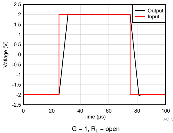
Figure 5-33. Large-Signal Step Response
