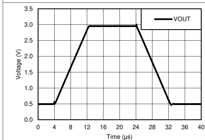
Figure 5-43. Voltage Follower Large Signal Response (50 pF)
